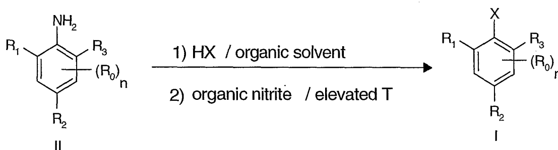
Reaction Scheme 1
