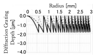
FIG.6I +1.5D&+3.0D Addition
