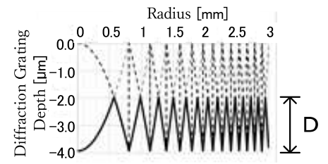
FIG.6C +1.5D&-1.5D Addition
