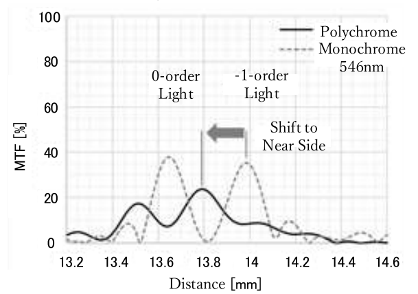
FIG.4C A=-1.5D , n=1.52
