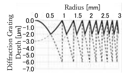
FIG.6L +2.0D&+1.0D&-1.0D Addition
