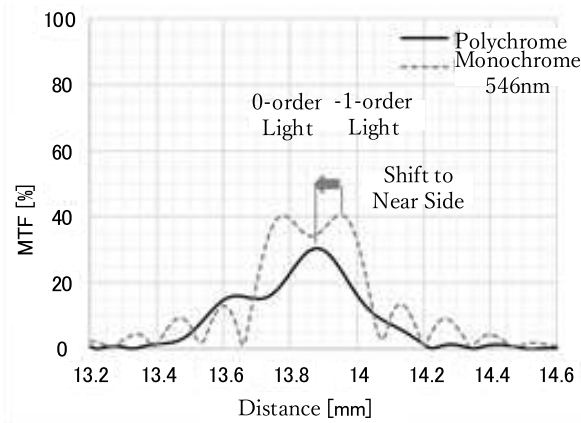
FIG.5C A=-0.75D , n=1.45
