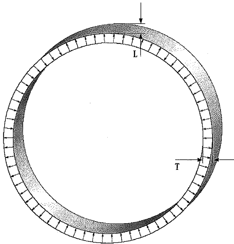
FIG. 3 (PRIOR ART)
