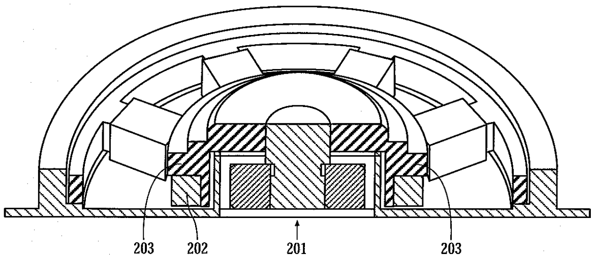
FIG. 2 (PRIOR ART)
