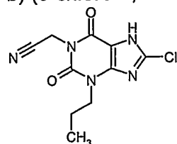
b) (8-chloro-2,6-dioxo-3-propyl-2,3,6,7-tetrahydro-1H-purin-1-yl)acetonitrile
