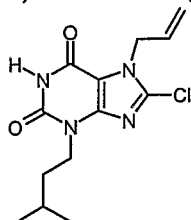
a) 8-chloro-3-(3-methylbutyl)-7-(2-propen-1-yl)-3,7-dihydro-1H-purine-2,6-dione
