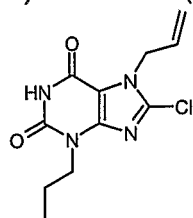
a) 8-chloro-7-(2-propen-1-yl)-3-propyl-3,7-dihydro-1H-purine-2,6-dione
