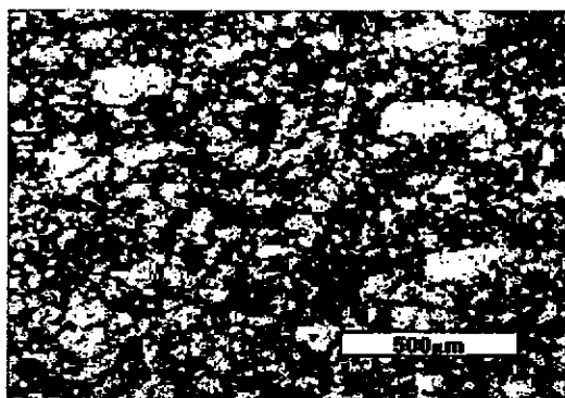
Fig. 2b: Microstructure of Al-30at%Ni-10at%Cr, Detail
