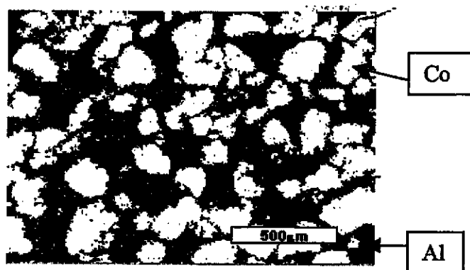
Fig. 2g: Microstructure of Co-50at%Al
