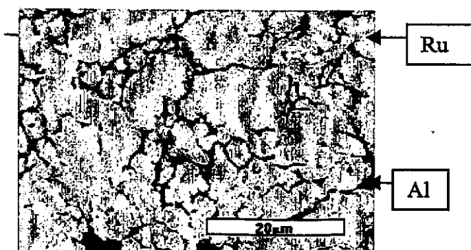
Fig. 2f: Microstructure of Ru-50at%Al, Detail
