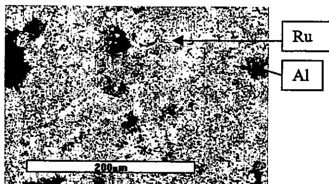
Fig. 2f: Microstructure of Ru-50at%Al, Detail
