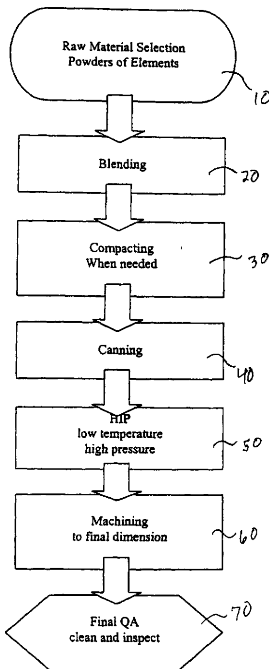
Figure 1. Process Flow Chart For Ductile Intermetallic Sputtering Targets
