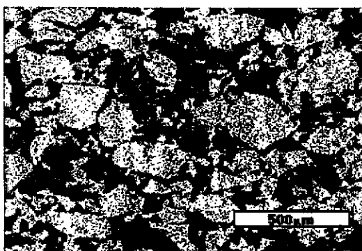
Fig. 2c: Microstructure of Ni-50at%Nb, Overview
