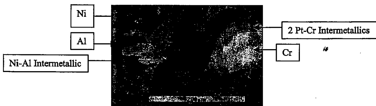
Fig. 2b: Microstructure of Al-30at%Ni-10at%Cr, Detail
