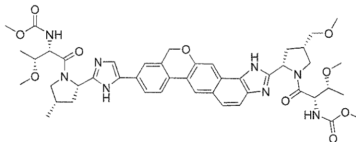
methyl {(2S,3R)-3-methoxy-1-[(2S,4S)-2-[9-(2-[(2S,4S)-1-[N-(methoxycarbonyl)-O-methyl-L-threonyl]-4-methylpyrrolidin-2-yl]-1H-imidazol-5-yl)-1,11-dihydroisochromeno[4',3':6,7]naphtho[1,2-d]imidazol-2-yl]-4-(methoxymethyl)pyrrolidin-1-yl]-1-oxobutan-2-yl}carbamate
