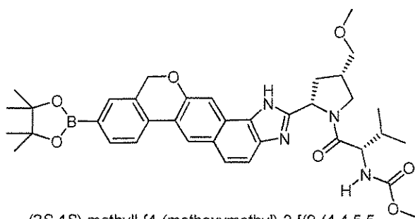
(2 S ,4 S )-methyl 4-(methoxymethyl)-2-[(9-(4,4,5,5-tetramethyl-1,3,2-dioxaborolan-2-yl)-1,11-dihydroisochromeno[4',3':6,7]naphtho[1,2-d]imidazol-2-yl)pyrrolidin-1-yl]-3-methyl-1-oxobutan-2-yl carbamate
