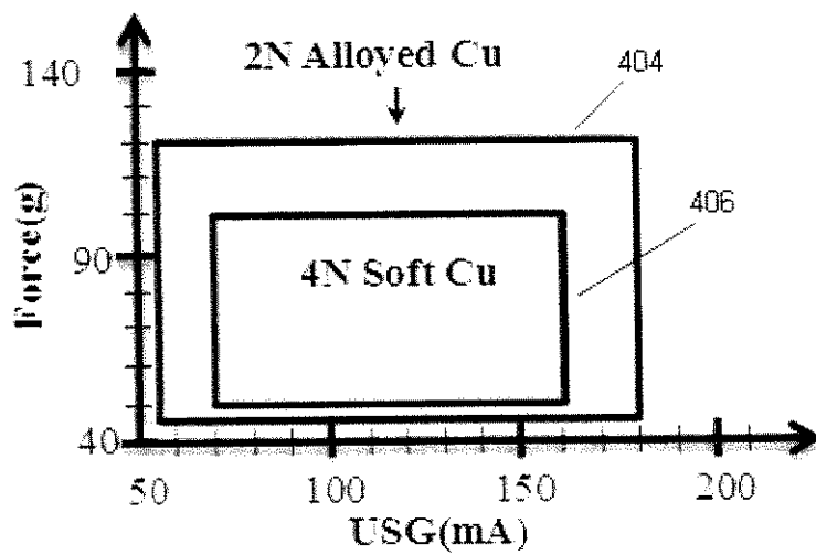
Fig 4(b) - Stitch Bond Process Window
