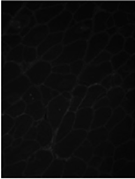
Figure 4A Untreated \beta -SG KO
