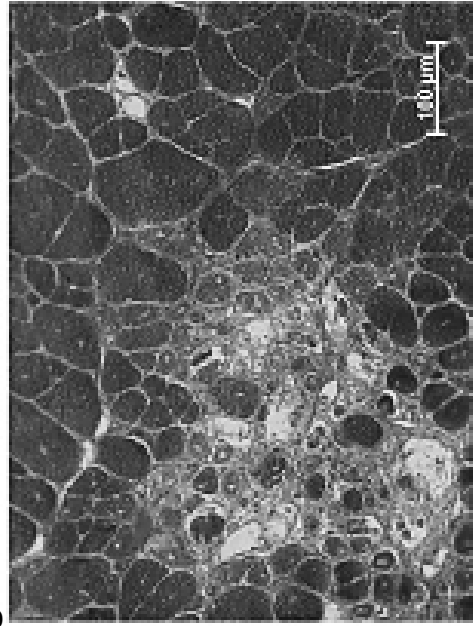
Figure 4B Untreated \beta -SG KO
