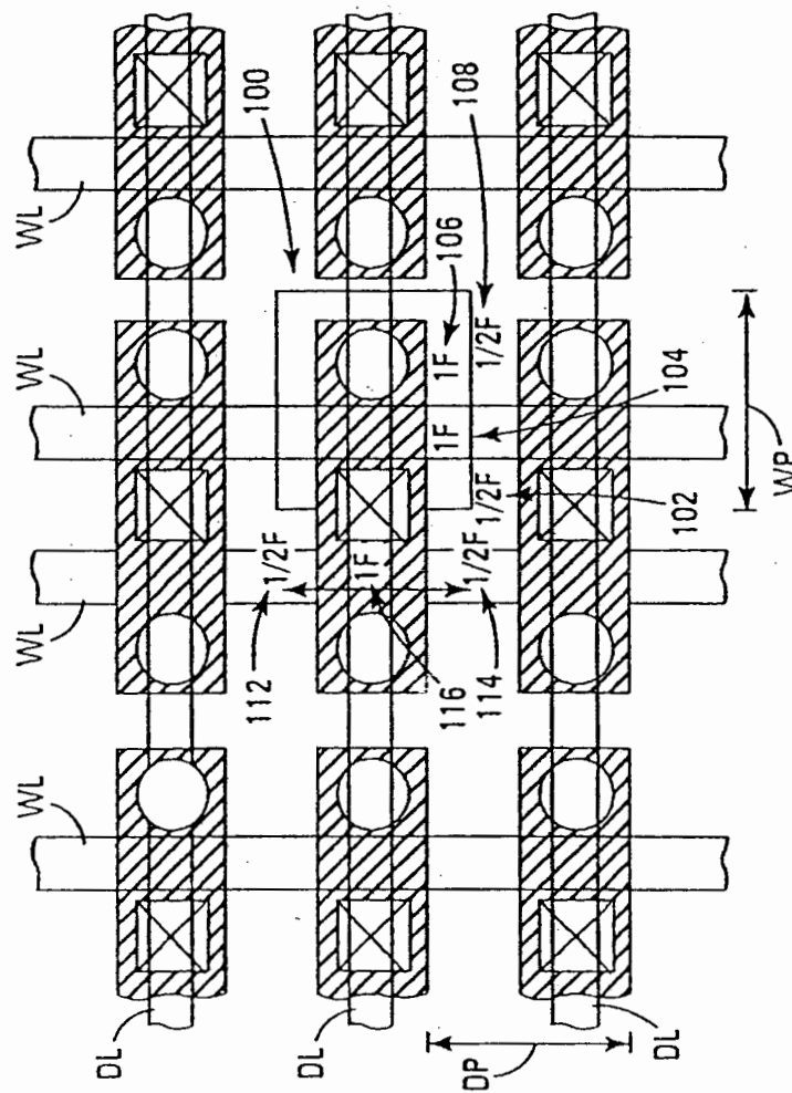
Fig. 2 Prior Art
