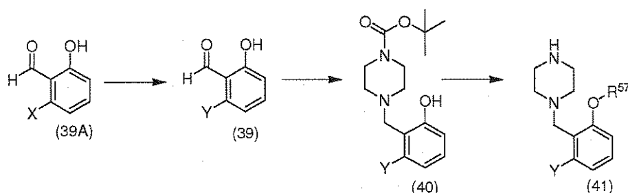
SCHEME 11
