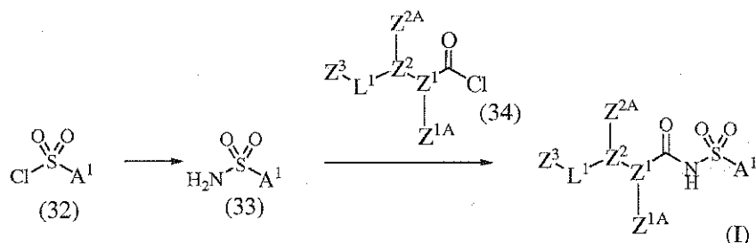
SCHEME 9
