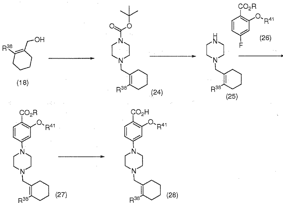
SCHEME 6
