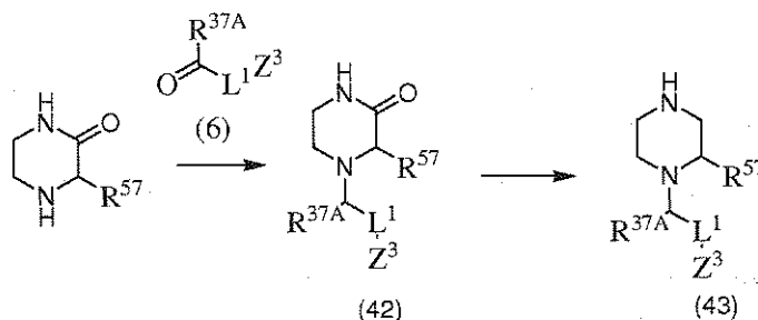
SCHEME 12
