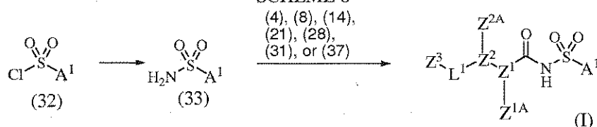
SCHEME 8
