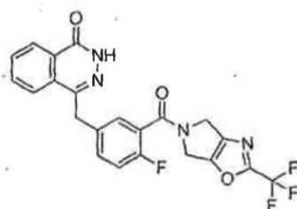
5 4-(3-(2-(cyclopropanecarbonyl)-5,6-dihydro-4H-pyrrolo[3,4-d]oxazole-5-carbonyl)-4-fluorobenzyl)phthalazin-1(2H)-one
