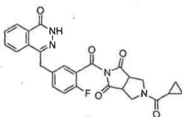
4-(4-fluoro-3-(2-(trifluoromethyl)-5,6-dihydro-4H-pyrrolo[3,4-d]oxazole-5-carbonyl)benzyl)phthalazin-1(2H)-one
