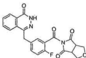
5-(2-fluoro-5-((4-oxo-3,4-dihydrophthalazin-1-yl)methyl)benzoyl)dihydro-1H-furo[3,4-c]pyrrole-4,6(5H,6aH)-dione
