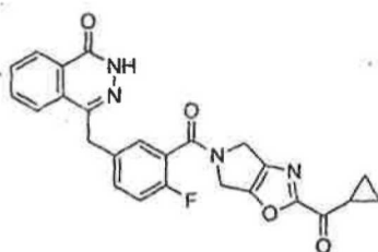
4-(4-fluoro-3-(2-(trifluoromethyl)-4,5,6,6a-tetrahydro-3aH-pyrrolo[3,4-d]thiazole-5-carbonyl)benzyl)phthalazin-1(2H)-one
