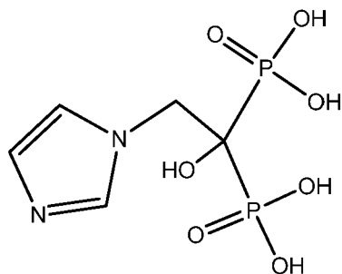
Zoledronic acid
