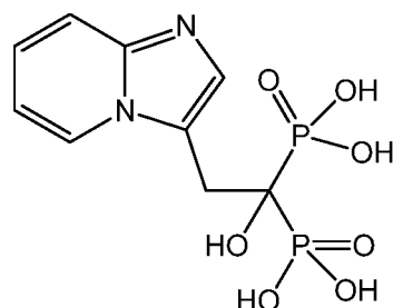
minodronic acid
