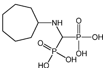
incadronic acid
