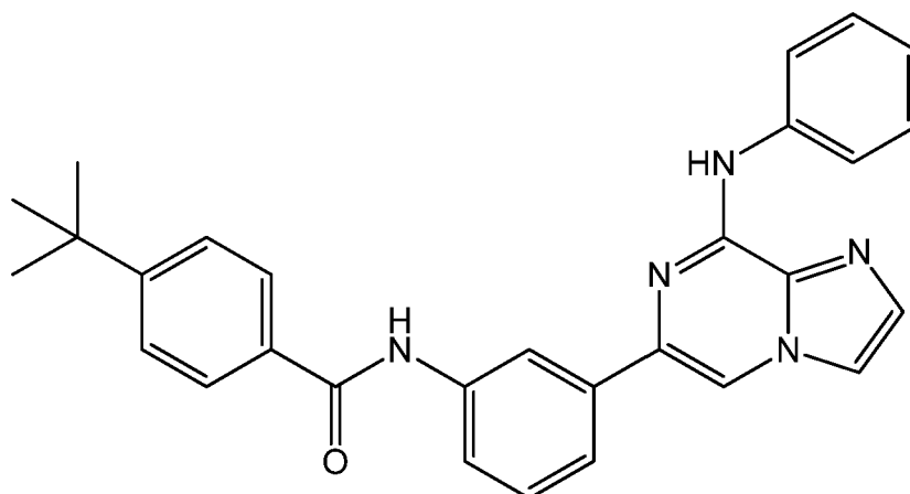
CGI-560
