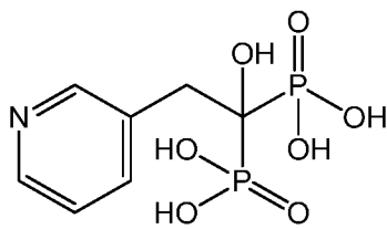
risedronic acid
