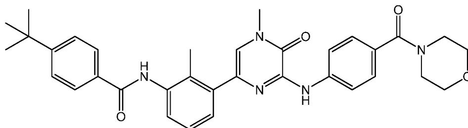
CGI-1746
