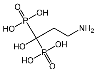
pamidronic acid
