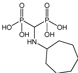
cimadronic acid
