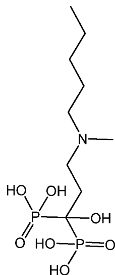
ibandronic acid
