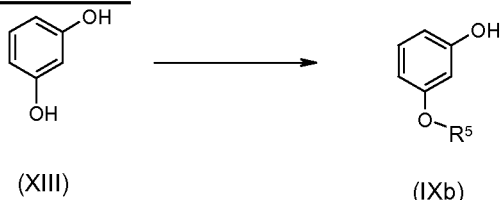
Scheme 9
