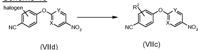
Scheme 16
