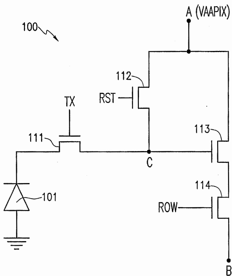
FIG. 1 (PRIOR ART)
