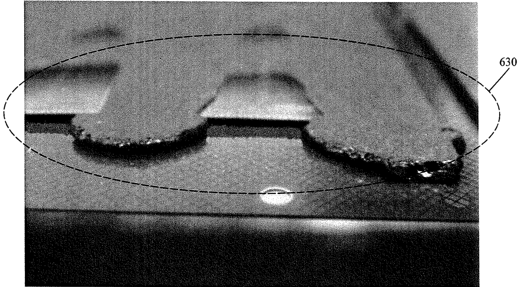
FIG. 6c (prior art)
