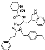
compound 138 N-((R)-1-(4-(4-ethylbenzyl)-5-phenethyl-4H-1,2,4-triazol-3-yl)-2-(1H-indol-3-yl)ethyl)picolinamide,
