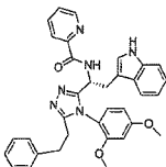
compound 160 N-((R)-2-(1H-indol-3-yl)-1-(4-(2,4-dimethoxyphenyl)-5-phenethyl-4H-1,2,4-triazol-3-yl)ethyl)-2-(pyridin-2-yl)acetamide,
