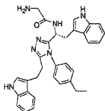
compound 150 (2S)-N-((R)-1-(5-(2-(1H-indol-3-yl)ethyl)-4-(4-ethylphenyl)-4H-1,2,4-triazol-3-yl)-2-(1H-indol-3-yl)ethyl)pyrrolidine-2-carboxamide,
