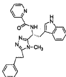
compound 175 N-((R)-1-(5-(2-(1H-indol-3-yl)ethyl)-4-phenyl-4H-1,2,4-triazol-3-yl)-2-(1H-indol-3-yl)ethyl)-2-amino-2-methylpropanamide,
