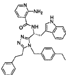
compound 140 (2S)-N-((R)-1-(4-(4-ethylbenzyl)-5-phenethyl-4H-1,2,4-triazol-3-yl)-2-(1H-indol-3-yl)ethyl)-2-aminopropanamide,
