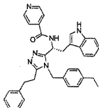
5 compound 142 N-((R)-2-(1H-indol-3-yl)-1-(5-phenethyl-4-phenyl-4H-1,2,4-triazol-3-yl)ethyl)piperidine-4-carboxamide,
