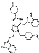
compound 46 (S)-N-((R)-1-(4-(4-methoxybenzyl)-5-phenethyl-4H-1,2,4-triazol-3-yl)-2-(1H-indol-3-yl)ethyl)pyrrolidine-2-carboxamide,
