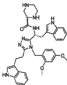
compound 73 (R)-N-(1-(5-(2-(1H-indol-3-yl)ethyl)-4-(2,4-dimethoxybenzyl)-4H-1,2,4-triazol-3-yl)-2-(1H-indol-3-yl)ethyl)picolinamide,
