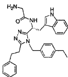
5 compound 136 N-((R)-1-(5-(2-(1H-indol-3-yl)ethyl)-4-(4-methoxybenzyl)-4H-1,2,4-triazol-3-yl)-2-(1H-indol-3-yl)ethyl)-2-(pyridin-4-yl)acetamide,
