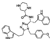
compound 82 (R)-N-(1-(4-(4-ethylbenzyl)-5-phenethyl-4H-1,2,4-triazol-3-yl)-2-(1H-indol-3-yl)ethyl)-2-(pyridin-2-yl)acetamide,
