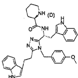
5 compound 89 (S)-N-((R)-1-(5-(2-(1H-indol-3-yl)ethyl)-4-(4-methoxybenzyl)-4H-1,2,4-triazol-3-yl)-2-(1H-indol-3-yl)ethyl)pyrrolidine-2-carboxamide,
