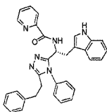
compound 147 N-((R)-1-(5-(2-(1H-indol-3-yl)ethyl)-4-(4-ethylphenyl)-4H-1,2,4-triazol-3-yl)-2-(1H-indol-3-yl)ethyl)picolinamide,
