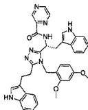
compound 72 (R)-N-1-(5-(2-(1H-indol-3-yl)ethyl)-4-(2,4-dimethoxybenzyl)-4H-1,2,4-triazol-3-yl)-2-(1H-indol-3-yl)ethyl)piperazine-2-carboxamide,
