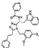
compound 66 (R)-N-(1-(4-(2,4-dimethoxybenzyl)-5-phenethyl-4H-1,2,4-triazol-3-yl)-2-(1H-indol-3-yl)ethyl)pyrazine-2-carboxamide,
