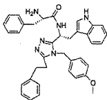
compound 187 ( R )-1-(5-(2-(1 H -indol-3-yl)ethyl)-4-(2,4-dimethoxybenzyl)-4 H -1,2,4-triazol-3-yl)-2-(1 H -indol-3-yl)- N -tosylethanamine,
