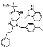
5 compound 44 (R)-N-(1-(4-(4-methoxybenzyl)-5-phenethyl-4H-1,2,4-triazol-3-yl)-2-(1H-indol-3-yl)ethyl)piperidine-4-carboxamide,
