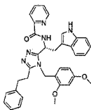
5 compound 65 (R)-N-(1-(4-(2,4-dimethoxybenzyl)-5-phenethyl-4H-1,2,4-triazol-3-yl)-2-(1H-indol-3-yl)ethyl)isonicotinamide,
