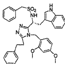
compound 177 (R)-1-(4-(2,4-dimethoxybenzyl)-5-phenethyl-4H-1,2,4-triazol-3-yl)-2-(1H-indol-3-yl)-N-phenylmethanesulfonylamine,
