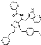
5 compound 139 N-((R)-1-(4-(4-ethylbenzyl)-5-phenethyl-4H-1,2,4-triazol-3-yl)-2-(1H-indol-3-yl)ethyl)-2-aminopyridine-3-carboxamide,
