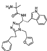
compound 182 N-((R)-1-(4-((furan-2-yl)methyl)-5-phenethyl-4H-1,2,4-triazol-3-yl)-2-(1H-indol-3-yl)ethyl)picolinamide,
