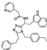
5 compound 155 (3S)-N-((R)-1-(4-(4-ethylbenzyl)-5-phenethyl-4H-1,2,4-triazol-3-yl)-2-(1H-indol-3-yl)ethyl)piperidine-3-carboxamide,
