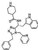
5 compound 167 N-((R)-1-(5-benzyl-4-((pyridin-4-yl)methyl)-4H-1,2,4-triazol-3-yl)-2-(1H-indol-3-yl)ethyl)-2-amino-2-methylpropanamide,
