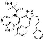
5 compound 34 (R)-N-(1-(5-(2-(1H-indol-3-yl)ethyl)-4-(4-methylbenzyl)-4H-1,2,4-triazol-3-yl)-2-(1H-indol-3-yl)ethyl)-2-amino-2-methylpropanamide,
