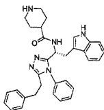
compound 143 (2S)-N-((R)-2-(1H-indol-3-yl)-1-(5-phenethyl-4-phenyl-4H-1,2,4-triazol-3-yl)ethyl)pyrrolidine-2-carboxamide,
