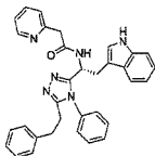
compound 146 N-((R)-2-(1H-indol-3-yl)-1-(5-phenethyl-4-phenyl-4H-1,2,4-triazol-3-yl)ethyl)picolinamide,
