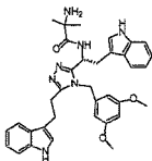
5 compound 22 (R)-N-(1-(4-(4-methoxybenzyl)-5-(3-phenylpropyl)-4H-1,2,4-triazol-3-yl)-2-(1H-indol-3-yl)ethyl)-2-amino-2-methylpropanamide,
