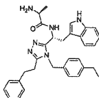
compound 141 N-((R)-1-(4-(4-ethylbenzyl)-5-phenethyl-4H-1,2,4-triazol-3-yl)-2-(1H-indol-3-yl)ethyl)isonicotinamide,
