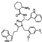
compound 87 (S)-N-((R)-1-(5-(2-(1H-indol-3-yl)ethyl)-4-(4-methoxybenzyl)-4H-1,2,4-triazol-3-yl)-2-(1H-indol-3-yl)ethyl)piperidine-3-carboxamide,
