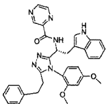
compound 162 N-((R)-2-(1H-indol-3-yl)-1-(4-(2,4-dimethoxyphenyl)-5-phenethyl-4H-1,2,4-triazol-3-yl)ethyl)-2-aminoacetamide,
