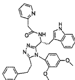
5 compound 161 N-((R)-2-(1H-indol-3-yl)-1-(4-(2,4-dimethoxyphenyl)-5-phenethyl-4H-1,2,4-triazol-3-yl)ethyl)pyrazine-2-carboxamide,
