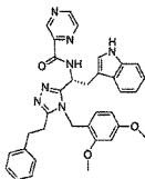
compound 67 (R)-N-1-(4-(2,4-dimethoxybenzyl)-5-phenethyl-4H-1,2,4-triazol-3-yl)-2-(1H-indol-3-yl)ethylpiperazine-2-carboxamide,
