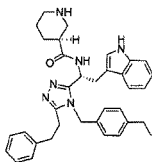
compound 156 N-((R)-1-(4-(4-ethylbenzyl)-5-phenethyl-4H-1,2,4-triazol-3-yl)-2-(1H-indol-3-yl)ethyl)-2-aminobenzamide,
