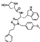
5 compound 41 (S)-N-((R)-1-(4-(4-methoxybenzyl)-5-phenethyl-4H-1,2,4-triazol-3-yl)-2-(1H-indol-3-yl)ethyl)piperidine-3-carboxamide,
