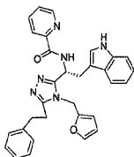
5 compound 183 N-((R)-1-(4-((furan-2-yl)methyl)-5-phenethyl-4H-1,2,4-triazol-3-yl)-2-(1H-indol-3-yl)ethyl)piperidine-4-carboxamide,
