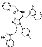
compound 149 N-((R)-1-(5-(2-(1H-indol-3-yl)ethyl)-4-(4-ethylphenyl)-4H-1,2,4-triazol-3-yl)-2-(1H-indol-3-yl)ethyl)-2-aminoacetamide,
