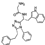
5 compound 145 N-((R)-2-(1H-indol-3-yl)-1-(5-phenethyl-4-phenyl-4H-1,2,4-triazol-3-yl)ethyl)-2-(pyridin-2-yl)acetamide,
