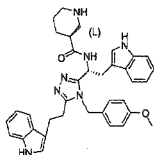
compound 88 (R)-N-((R)-1-(5-(2-(1H-indol-3-yl)ethyl)-4-(4-methoxybenzyl)-4H-1,2,4-triazol-3-yl)-2-(1H-indol-3-yl)ethyl)piperidine-2-carboxamide,
