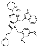
compound 64 (R)-N-(1-(4-(2,4-dimethoxybenzyl)-5-phenethyl-4H-1,2,4-triazol-3-yl)-2-(1H-indol-3-yl)ethyl)picolinamide,
