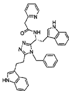
compound 61 (R) -N-(1-(5-(2-(1 H -indol-3-yl)ethyl)-4-(2,4-dimethoxybenzyl)-4 H -1,2,4-triazol-3-yl)-2-(1 H -indol-3-yl)ethyl)-2-(pyridin-2-yl)acetamide,
