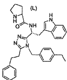
compound 135 N-((R)-1-(4-(4-ethylbenzyl)-5-phenethyl-4H-1,2,4-triazol-3-yl)-2-(1H-indol-3-yl)ethyl)-2-aminoacetamide,
