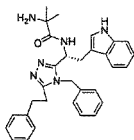
compound 174 N -(( R )-2-(1 H -indol-3-yl)-1-(4-methyl-5-phenethyl-4 H -1,2,4-triazol-3-yl)ethyl)picolinamide,
