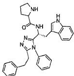
compound 144 N-((R)-2-(1H-indol-3-yl)-1-(5-phenethyl-4-phenyl-4H-1,2,4-triazol-3-yl)ethyl)-2-aminoacetamide,
