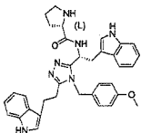
compound 90 (R)-N-((R)-1-(5-(2-(1H-indol-3-yl)ethyl)-4-(4-methoxybenzyl)-4H-1,2,4-triazol-3-yl)-2-(1H-indol-3-yl)ethyl)pyrrolidine-2-carboxamide,
