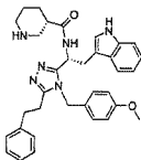
compound 42 (R)-N-((R)-1-(4-(4-methoxybenzyl)-5-phenethyl-4H-1,2,4-triazol-3-yl)-2-(1H-indol-3-yl)ethyl)piperidine-3-carboxamide,
