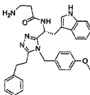
compound 57 (S)-N-((R)-1-(4-(4-methoxybenzyl)-5-phenethyl-4H-1,2,4-triazol-3-yl)-2-(1H-indol-3-yl)ethyl)-2-aminopropanamide,
