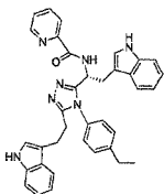
5 compound 148 N-((R)-1-(5-(2-(1H-indol-3-yl)ethyl)-4-(4-ethylphenyl)-4H-1,2,4-triazol-3-yl)-2-(1H-indol-3-yl)ethyl)-2-(pyridin-2-yl)acetamide,
