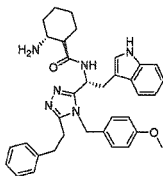
compound 154 N-((R)-1-(4-(4-ethylbenzyl)-5-phenethyl-4H-1,2,4-triazol-3-yl)-2-(1H-indol-3-yl)ethyl)-2-(pyridin-3-yl)acetamide,
