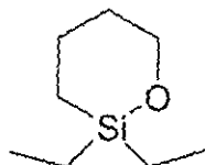
2,2-dipropyl-1-oxa-2-silacyclohexane
