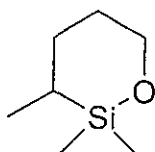
5 2,2,3-trimethyl-1-oxa-2-silacyclohexane
