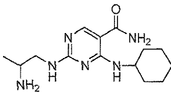
2-(2-amino-2-oxoethylamino)-4-(cyclohexylamino)pyrimidine-5-carboxamide
