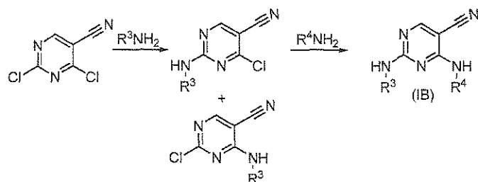
Scheme 8
