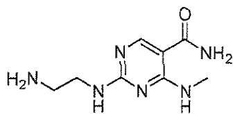
2-(2-aminopropylamino)-4-(cyclohexylamino)pyrimidine-5-carboxamide
