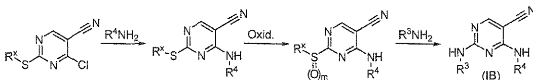
Scheme 9
