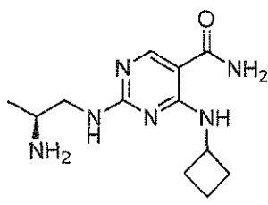
(S)-2-(2-aminopropylamino)-4-(cyclobutylamino)pyrimidine-5-carboxamide
