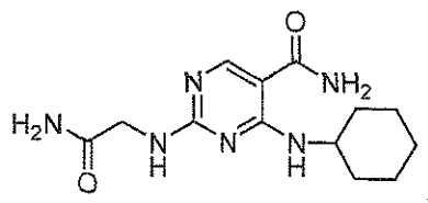
2-(2-aminoethylamino)-4-(cyclohexylamino)pyrimidine-5-carboxamide
