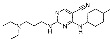
2-(3-(diethylamino)propylamino)-4-(4-methylcyclohexylamino)pyrimidine-5-carbonitrile
