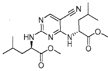
(2S,2'S)-diethyl 2,2'-(5-cyanopyrimidine-2,4-diyl)bis(azanediy)-bis(3-methylbutanoate)
