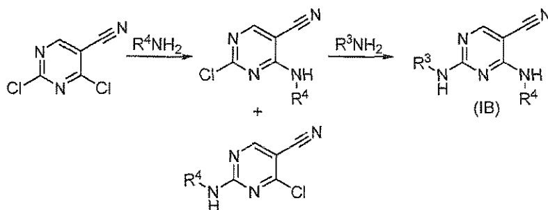
Scheme 7
