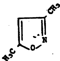
3,5-dimethylisoxazole
