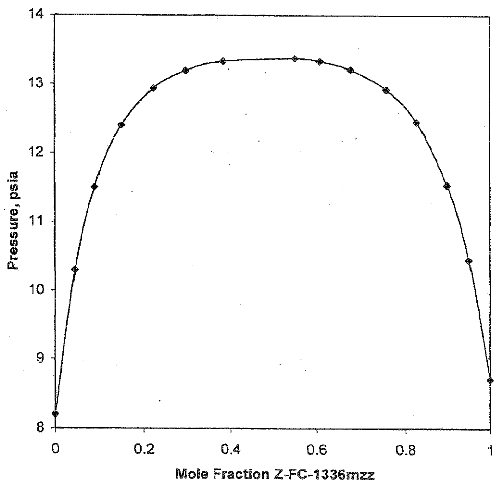
FIGURE 2. Z-FC-1336mzz and n-Pentane at 19.9 C
