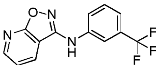
N-(3-(trifluoromethyl)phenyl)isoxazolo[5,4-b]pyridin-3-amine
