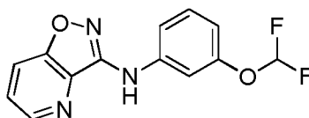
N-(3-(difluoromethoxy)phenyl)isoxazolo[4,5-b]pyridin-3-amine
