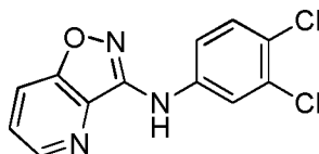
N-(3,4-dichlorophenyl)isoxazolo[4,5-b]pyridin-3-amine
