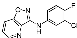
N-(3-chloro-4-fluorophenyl)isoxazolo[4,5-b]pyridin-3-amine
