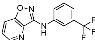
N-(3-(trifluoromethyl)phenyl)isoxazolo[4,5-b]pyridin-3-amine
