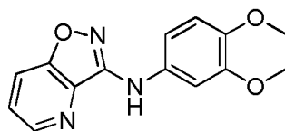
N-(3,4-dimethoxyphenyl)isoxazolo[4,5-b]pyridin-3-amine
