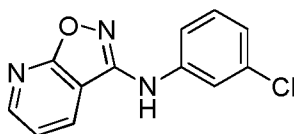
N-(3-chlorophenyl)isoxazolo[5,4-b]pyridin-3-amine
