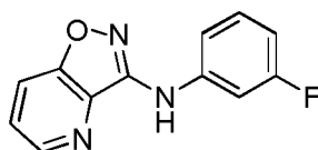
N-(3-fluorophenyl)isoxazolo[4,5-b]pyridine-3-amine
