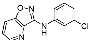
N-(3-chlorophenyl)isoxazolo[4,5-b]pyridin-3-amine
