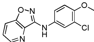
N-(3-chloro-4-methoxyphenyl)isoxazolo[4,5-b]pyridin-3-amine
