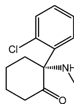
( R )-ketamine
