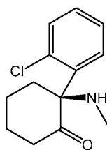
( S )-ketamine
