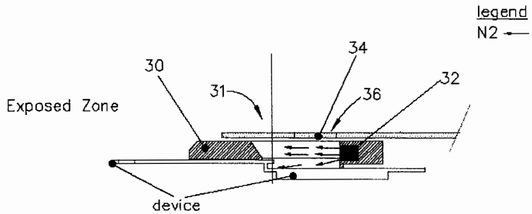
Figure 5 – Bonding area
