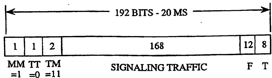
FIG. 2e BLANK AND BURST WITH SIGNALING TRAFFIC ONLY (9.6 KBPS)
