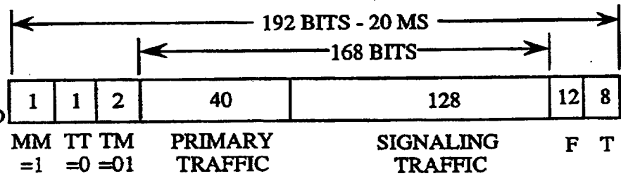
FIG. 2c DIM AND BURST WITH RATE 1/4 PRIMARY AND SIGNALING TRAFFIC (9.6 KBPS)
