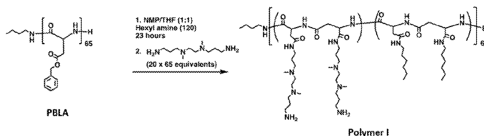
Scheme 15: Synthesis of Polymer I
