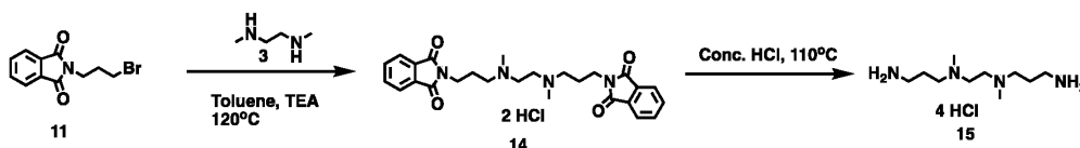
Scheme 14: Synthesis of Amine Compound 15
