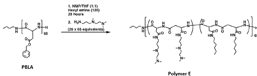
Scheme 8: Synthesis of Polymer E
