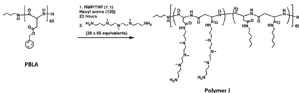
Scheme 17: Synthesis of Polymer J
