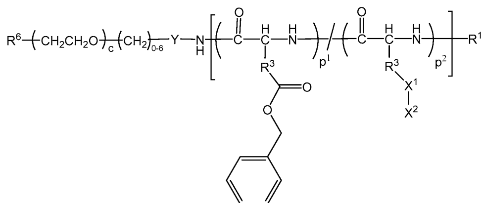
Formula 3A
