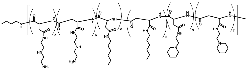
Polymer 47
