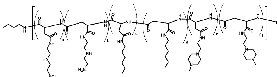
Polymer 49
