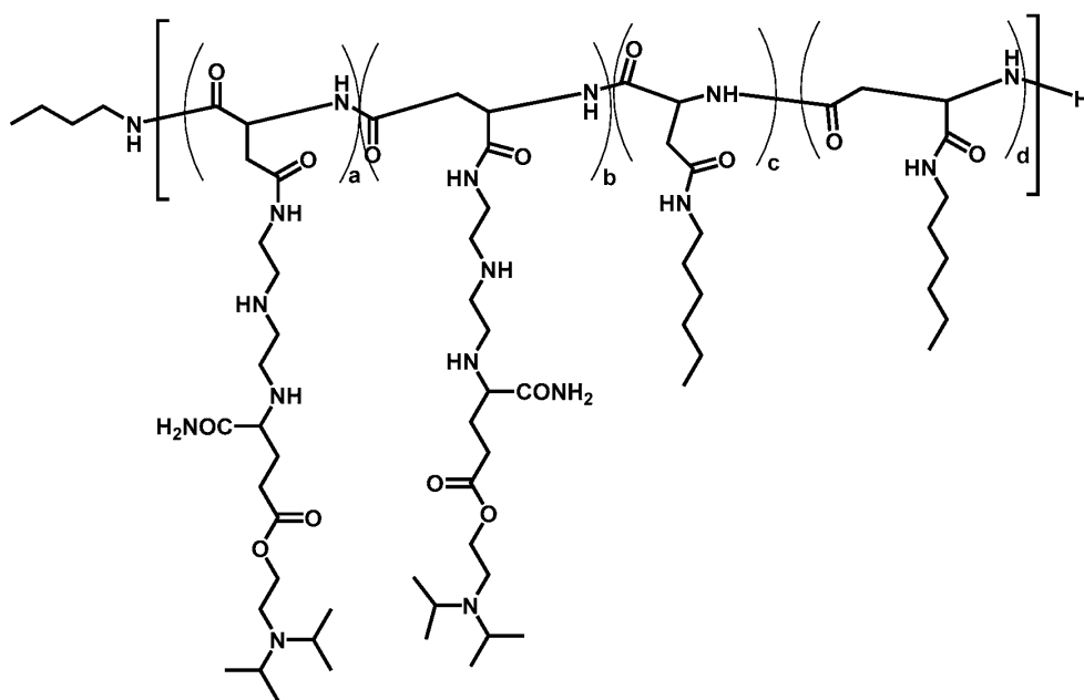
Polymer 67
