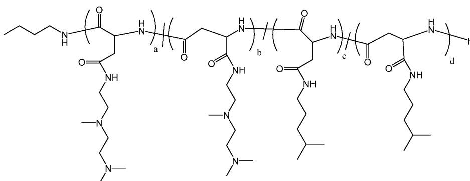
Polymer 35
