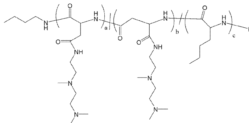
Polymer 21
