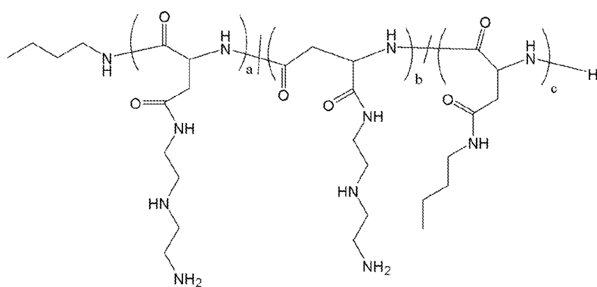
Polymer 7
