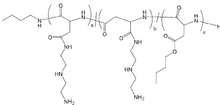
Polymer 8
