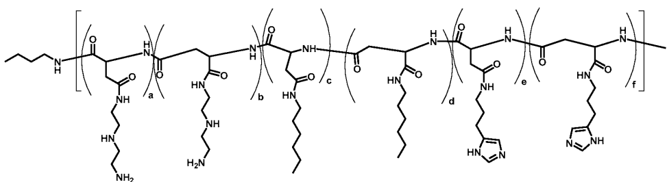
Polymer 59
