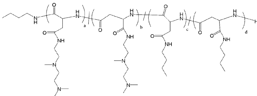
Polymer 27
