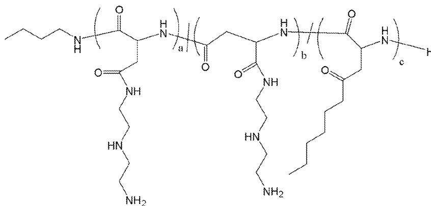
Polymer 2
