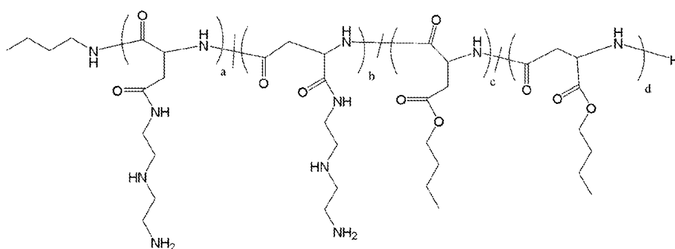
Polymer 12
