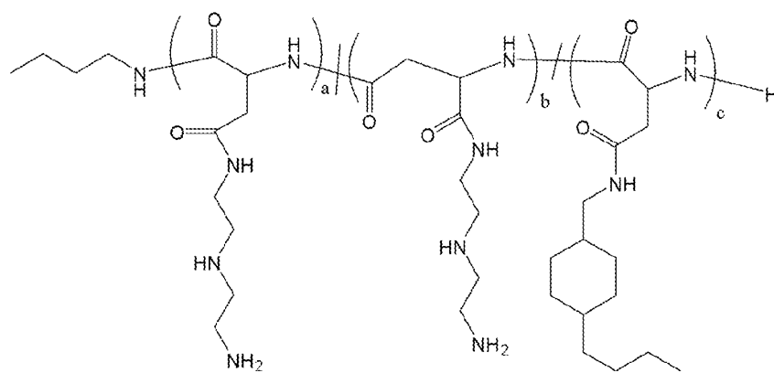
Polymer 9
