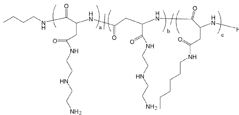
Polymer 3
