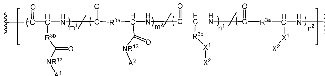
Formula 4
