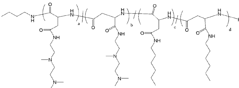
Polymer 29
