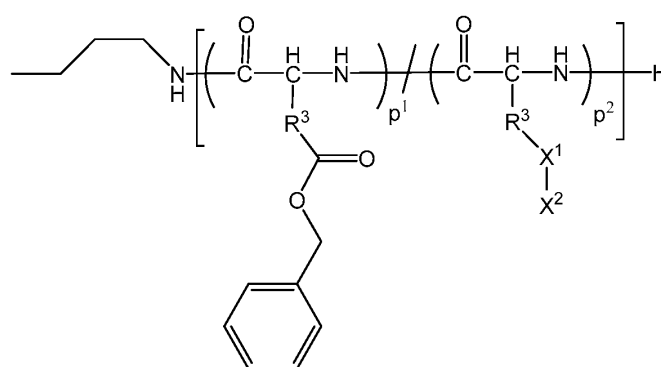
Formula 3B
