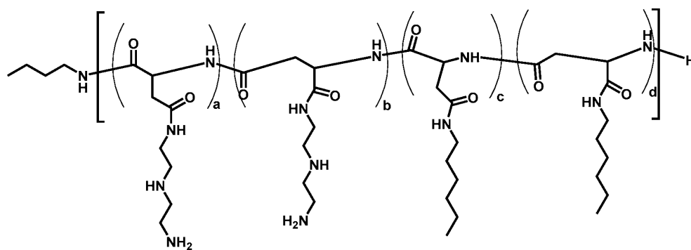
Polymer 37
