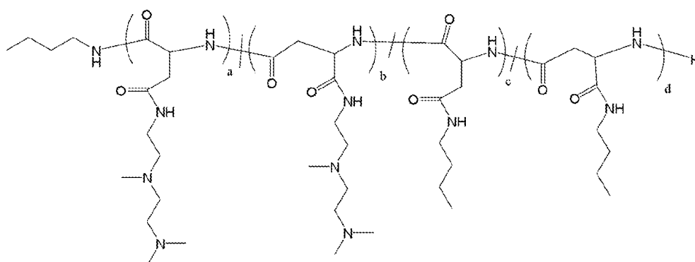
Polymer 27
