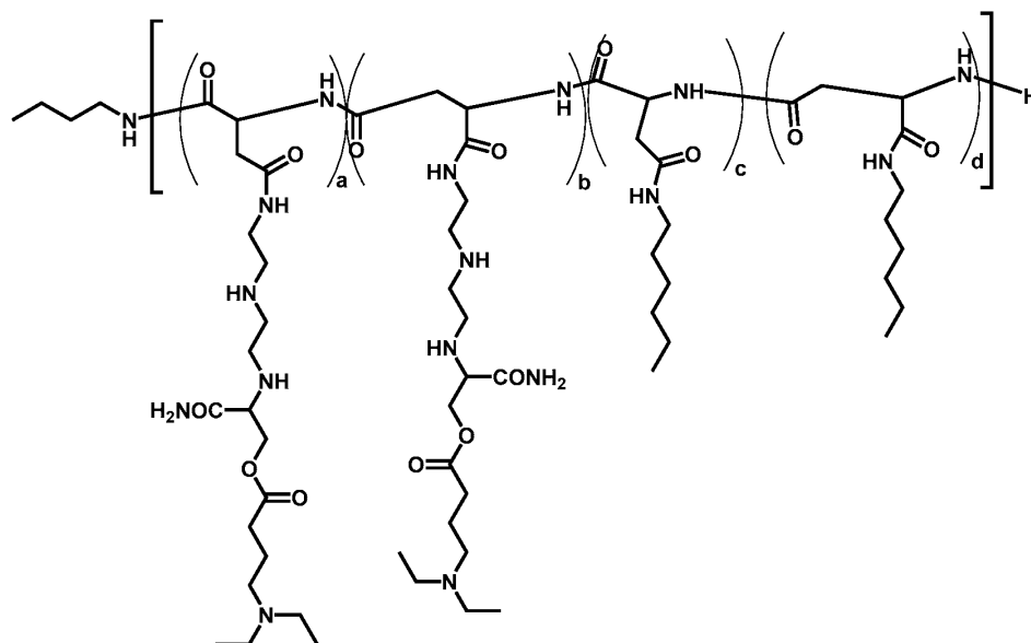
Polymer 61
