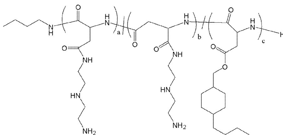
Polymer 10
