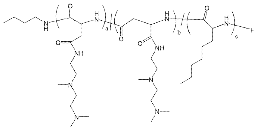
Polymer 17
