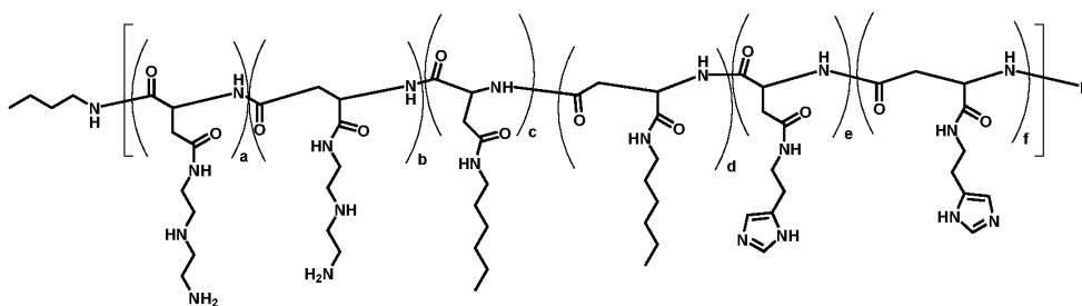
Polymer 51
