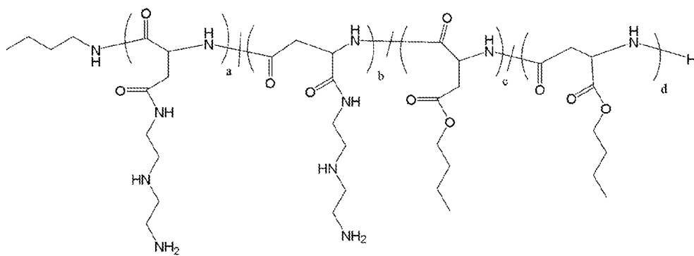
Polymer 12
