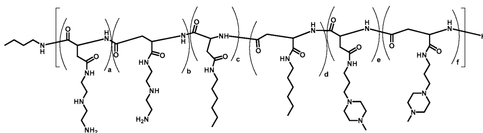
Polymer 57
