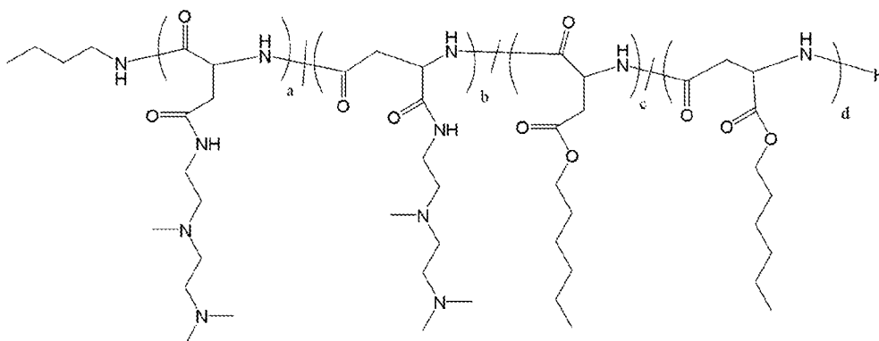
Polymer 30
