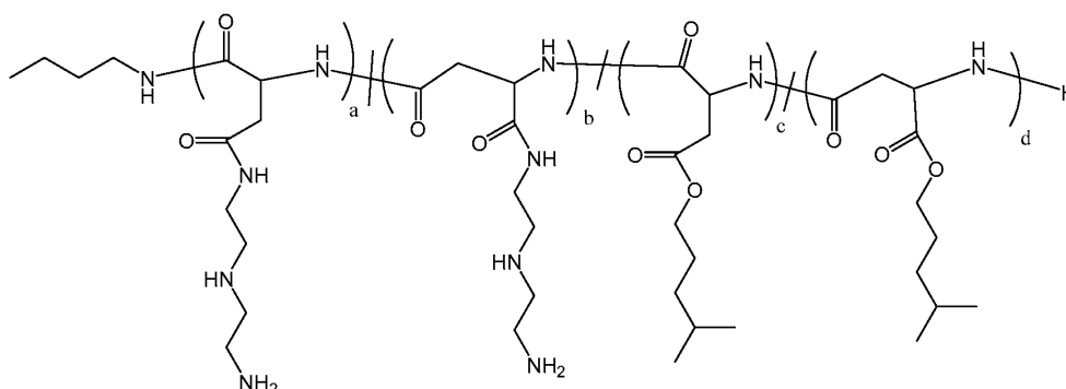
Polymer 34
