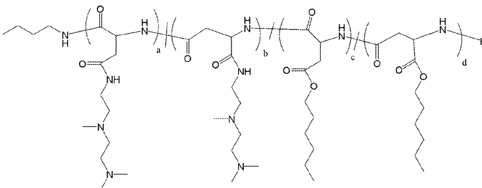
Polymer 30
