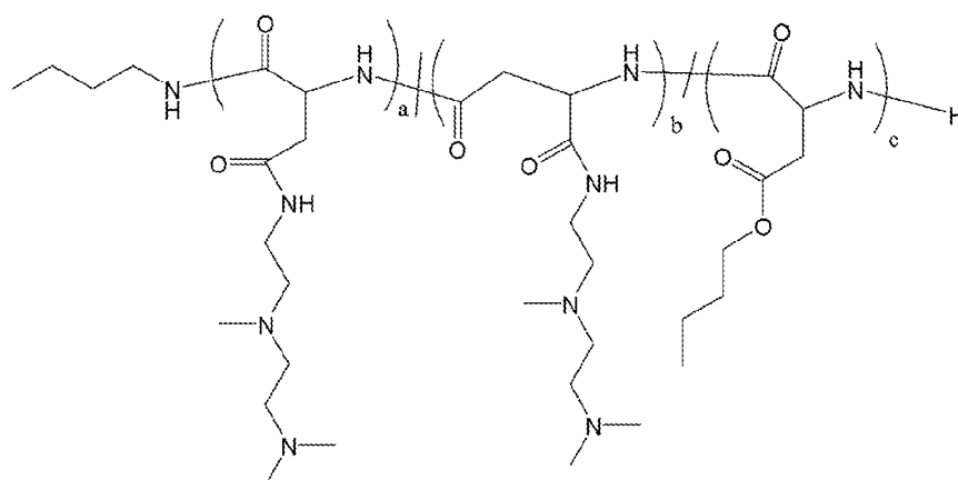
Polymer 24
