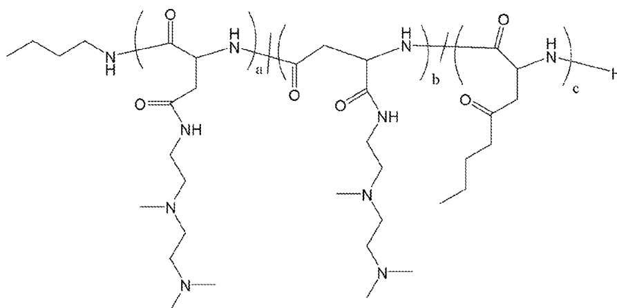
Polymer 22
