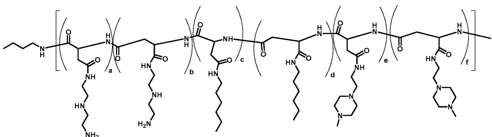
Polymer 49
