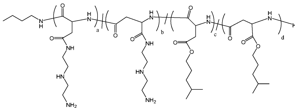
Polymer 34
