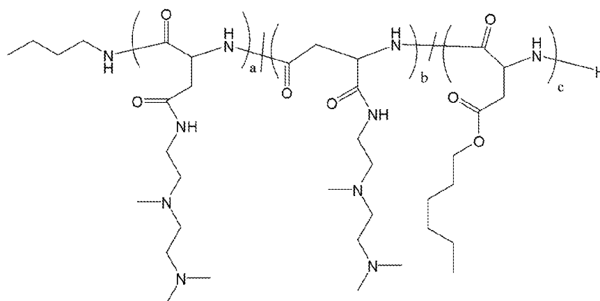
Polymer 20
