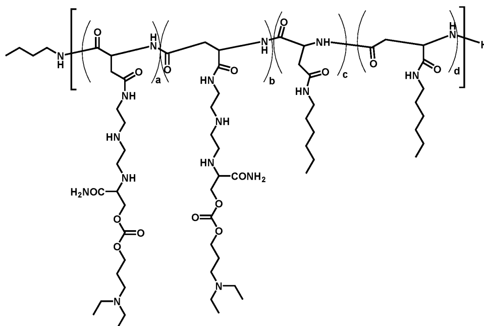
Polymer 62
