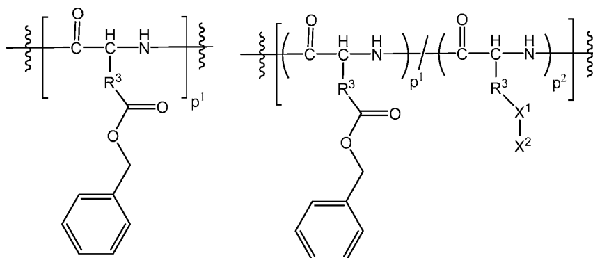
Formula 2
