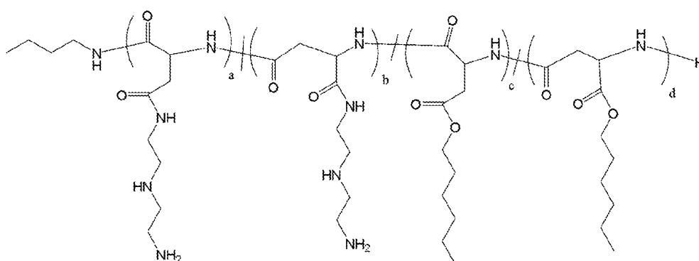
Polymer 14
