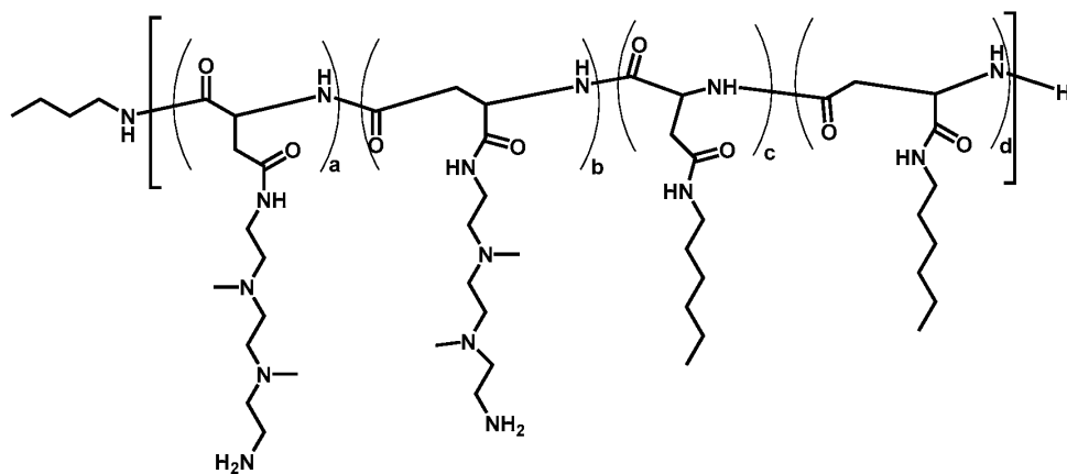
Polymer 41
