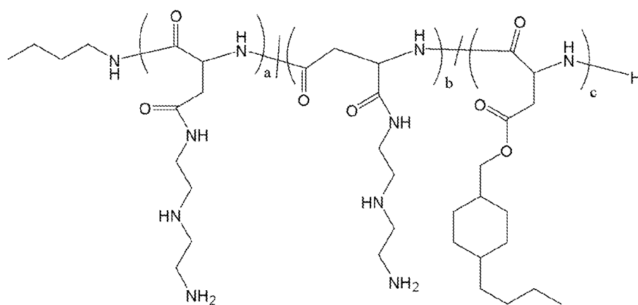
Polymer 10
