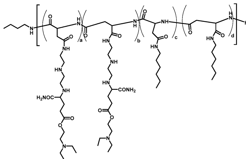
Polymer 63
