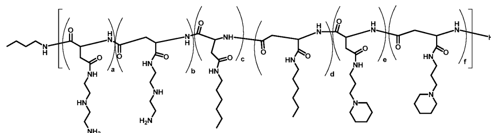
Polymer 55
