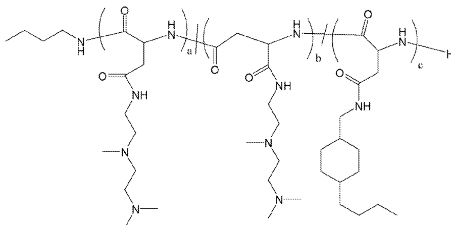
Polymer 25
