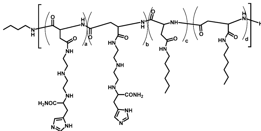
Polymer 60
