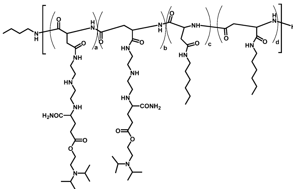
Polymer 67
