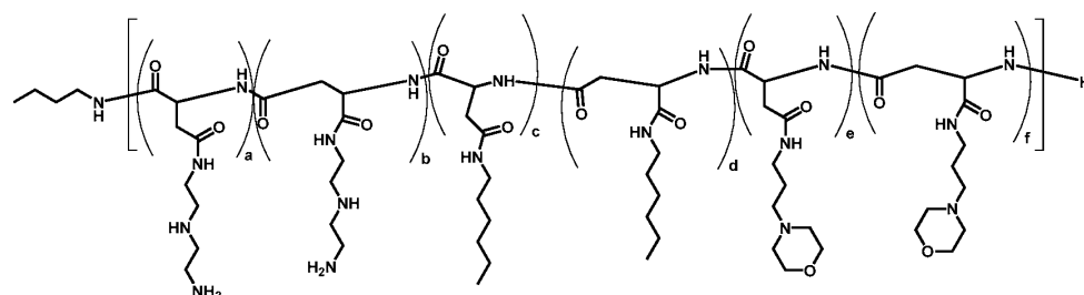
Polymer 56
