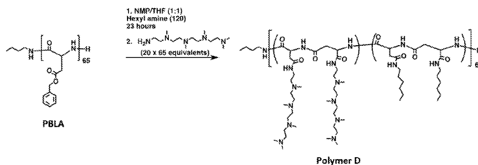
Scheme 6: Synthesis of Polymer D:
