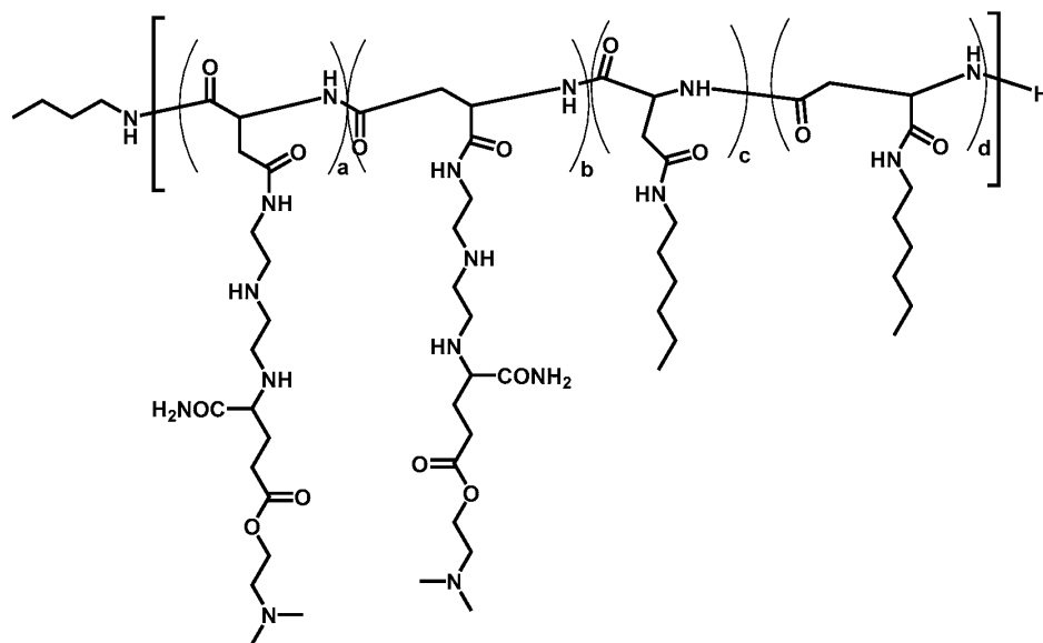
Polymer 66
