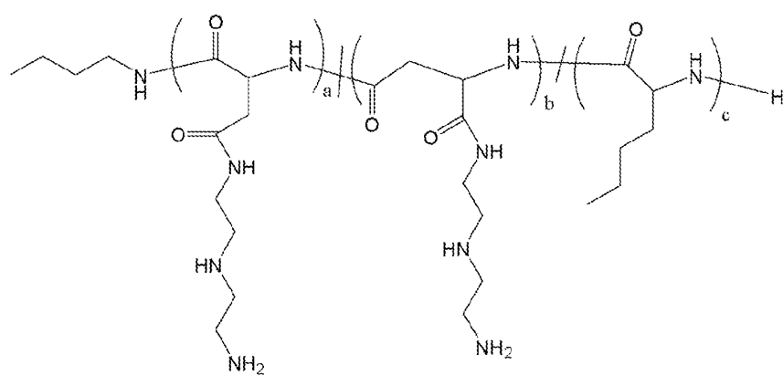
Polymer 5
