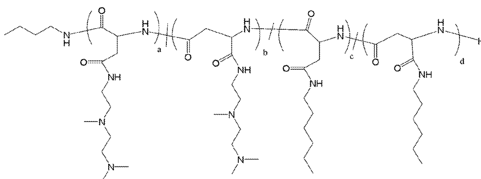
Polymer 29
