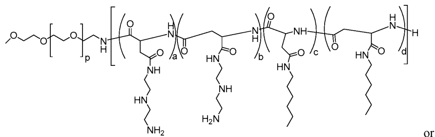
Polymer 68
