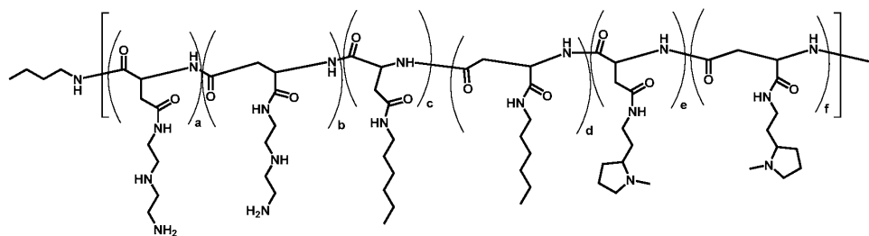
Polymer 50
