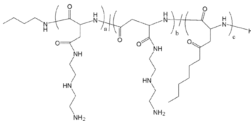
Polymer 2
