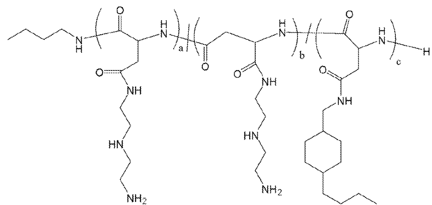
Polymer 9
