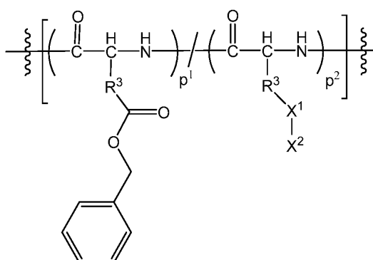
Formula 3
