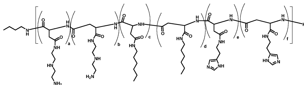
Polymer 51
