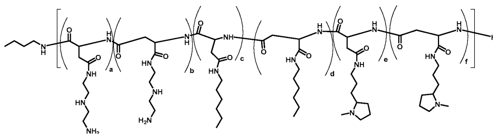
Polymer 58
