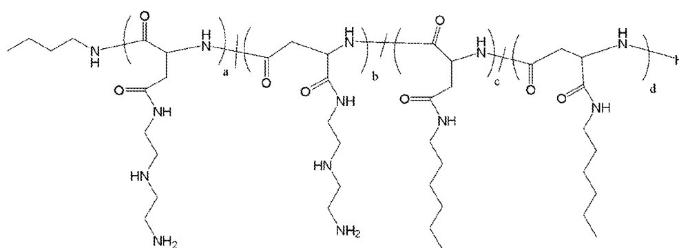
Polymer 13
