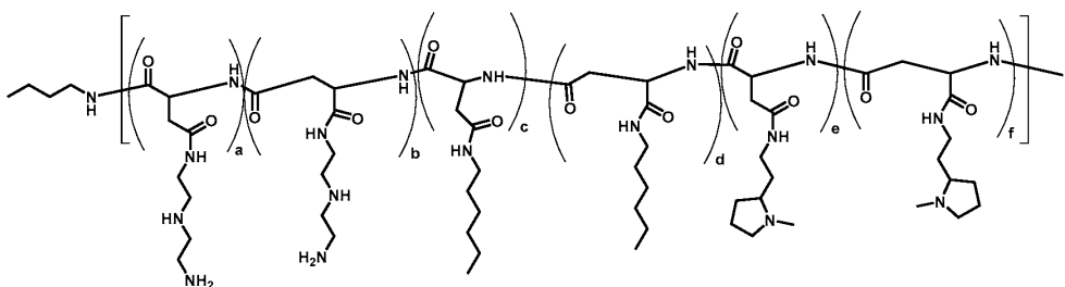
Polymer 50
