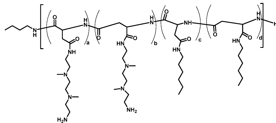
Polymer 41
