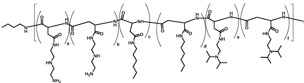
Polymer 46
