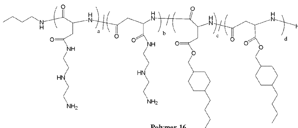
Polymer 16
