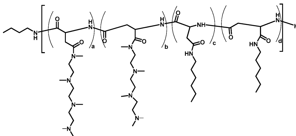
Polymer 38
