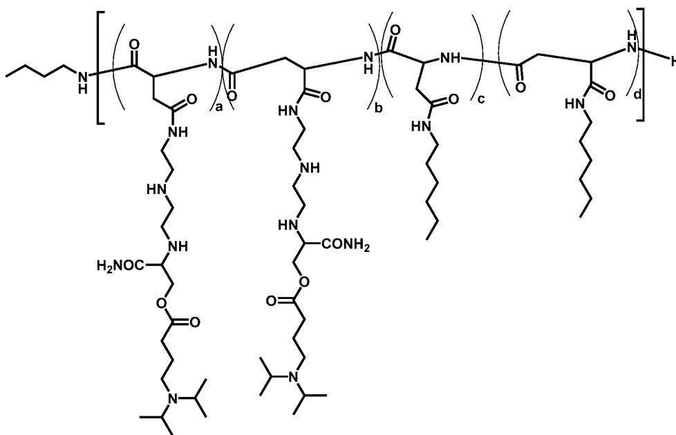
Polymer 65
