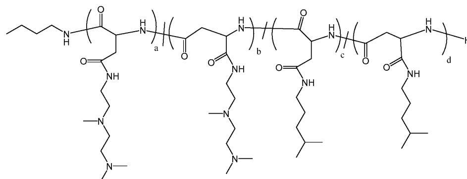
Polymer 35
