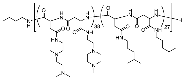
Polymer C
