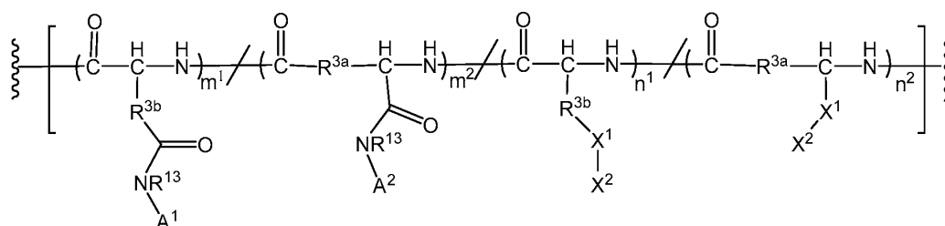
Formula 4
