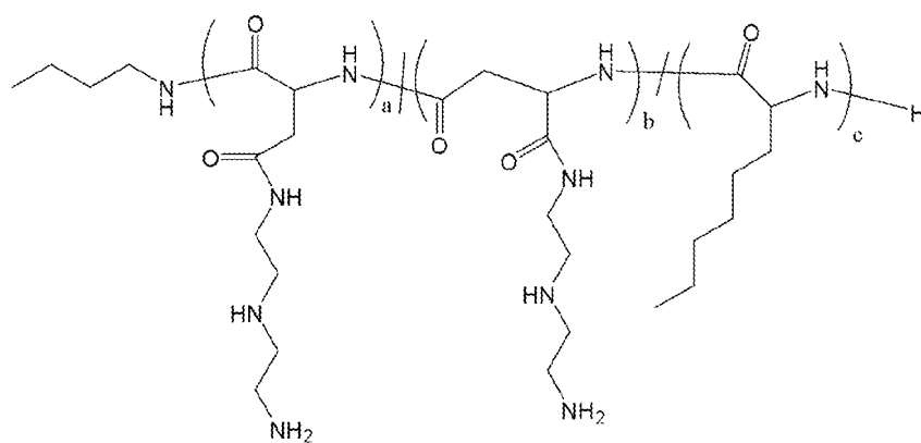
Polymer 1
