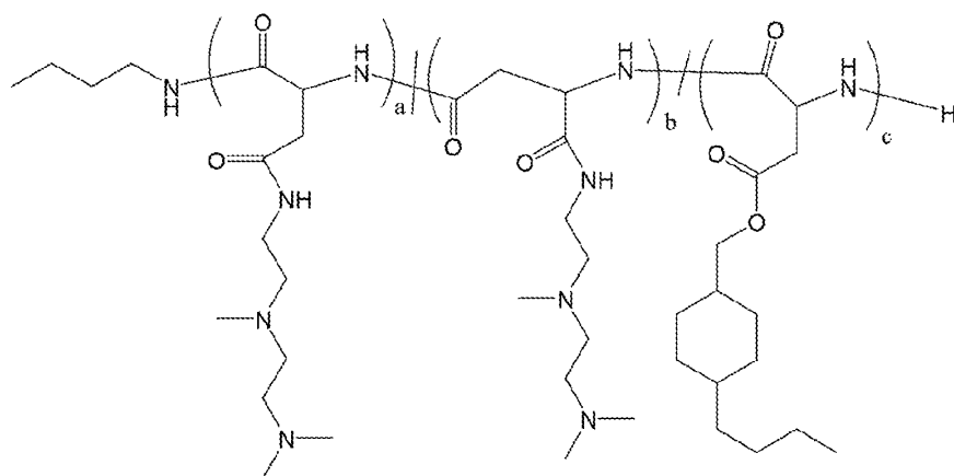
Polymer 26
