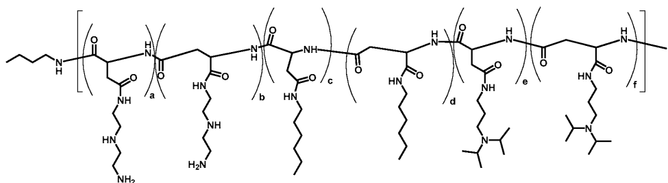
Polymer 54
