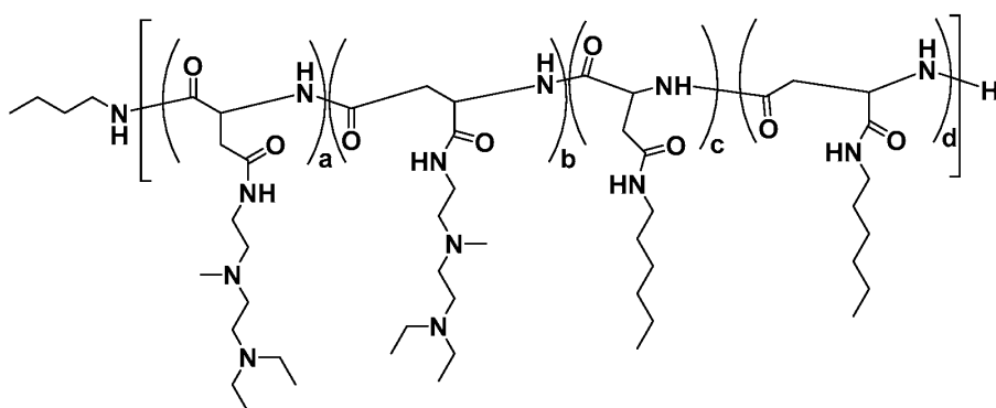
Polymer 43
