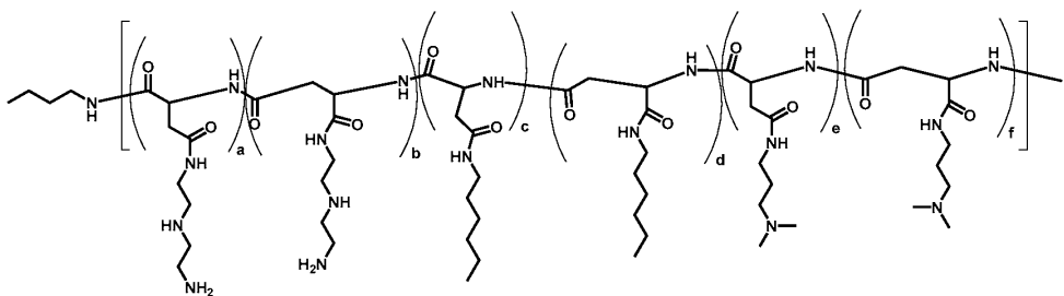
Polymer 52
