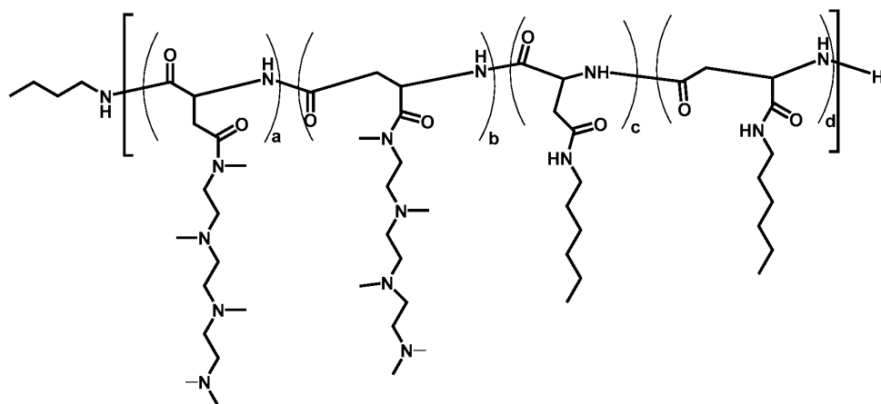
Polymer 38
