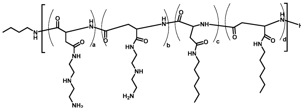
Polymer 37
