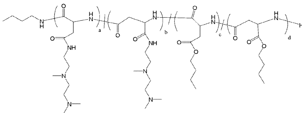
Polymer 28
