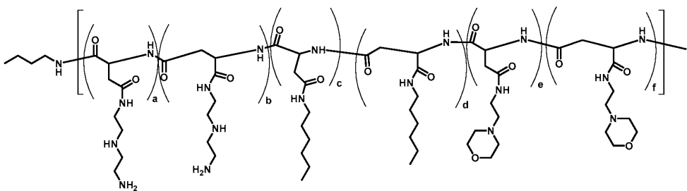
Polymer 48
