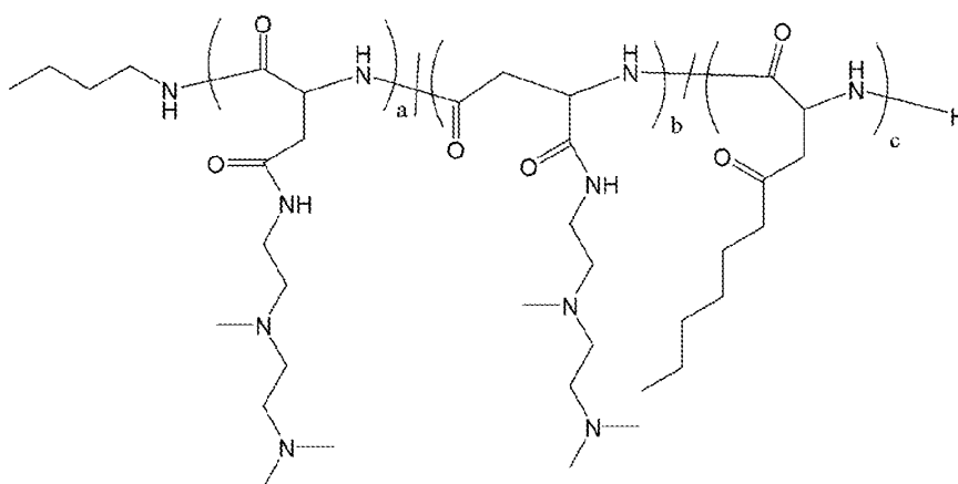
Polymer 18
