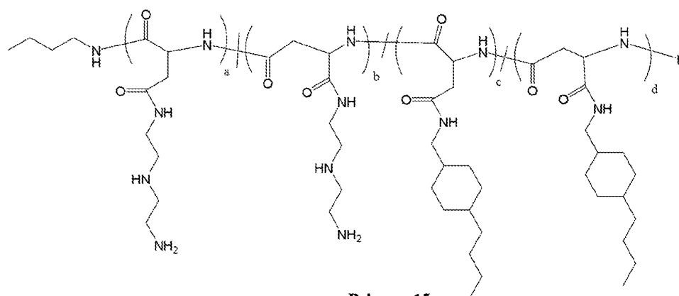
Polymer 15
