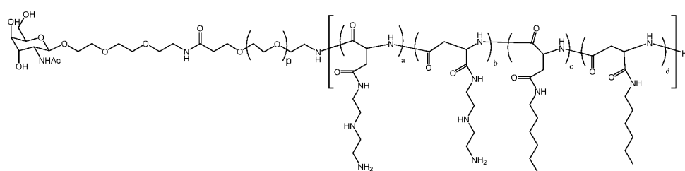
Polymer 69
