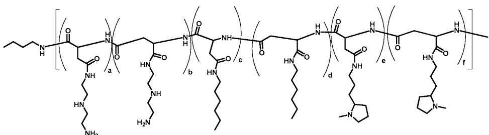
Polymer 58
