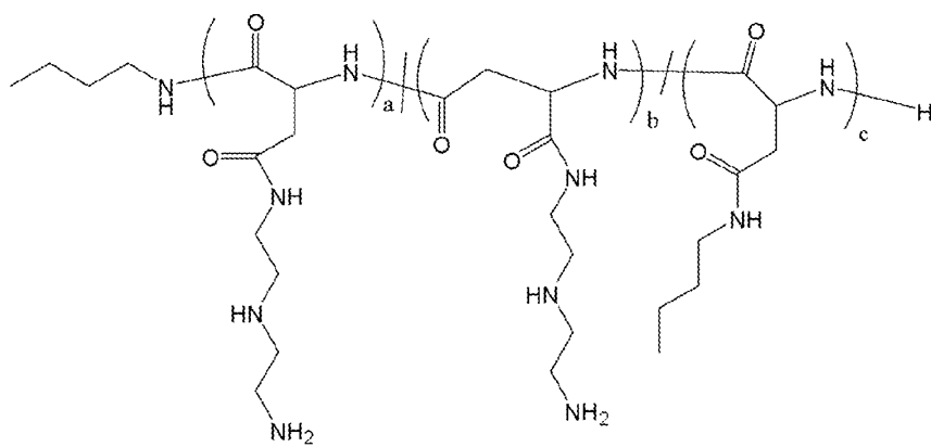
Polymer 7
