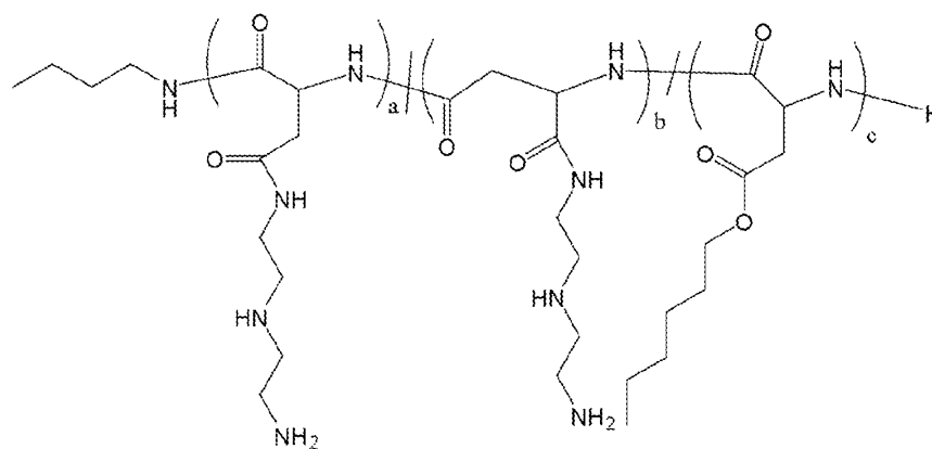
Polymer 4
