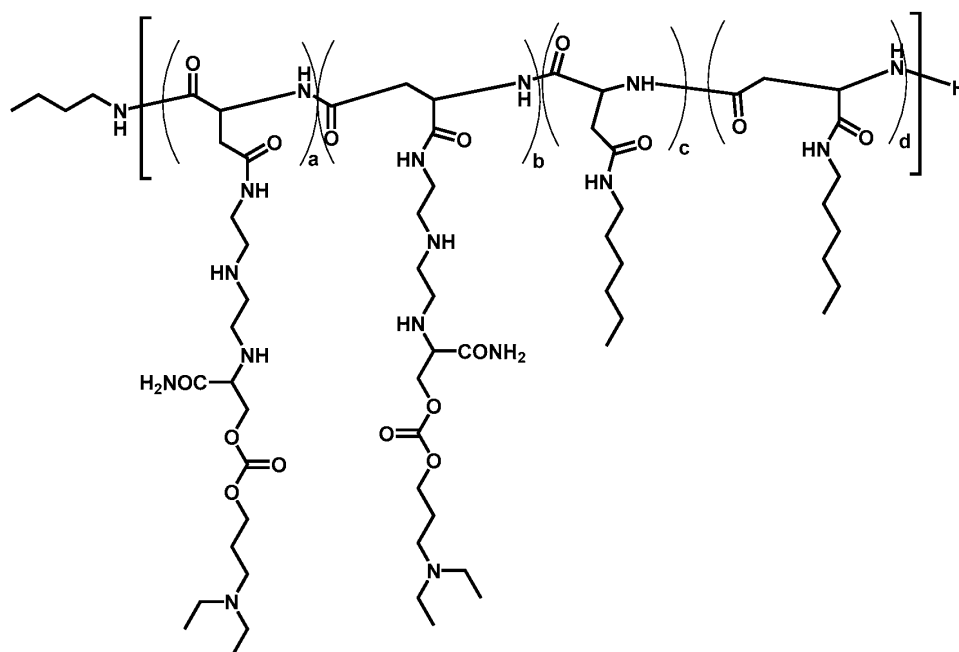
Polymer 62
