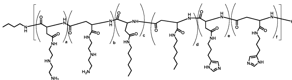
Polymer 59
