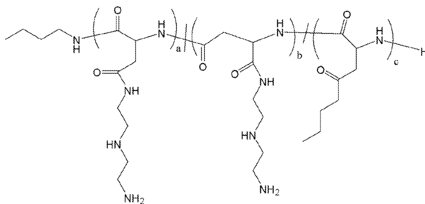
Polymer 6
