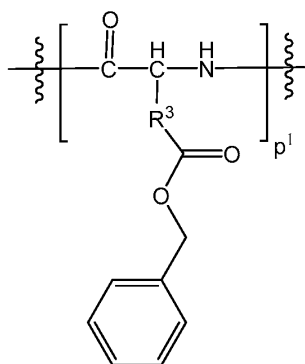
Formula 2
