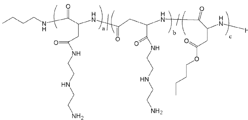
Polymer 8
