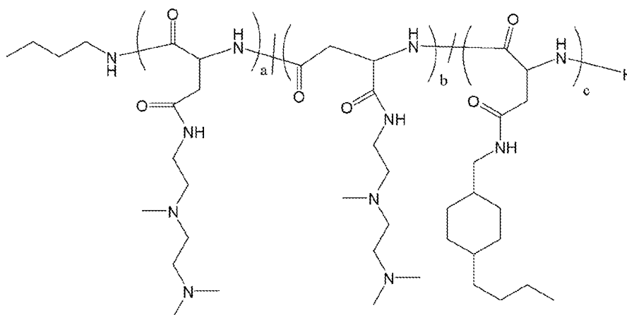
Polymer 25
