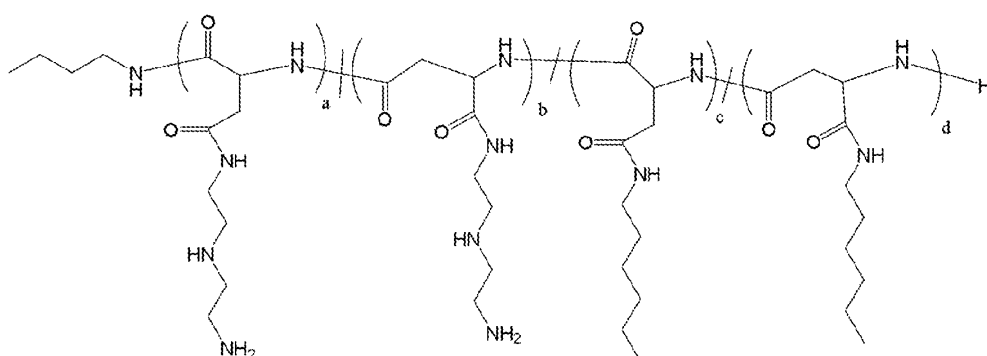
Polymer 13
