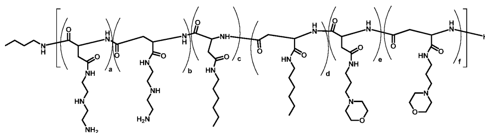
Polymer 56
