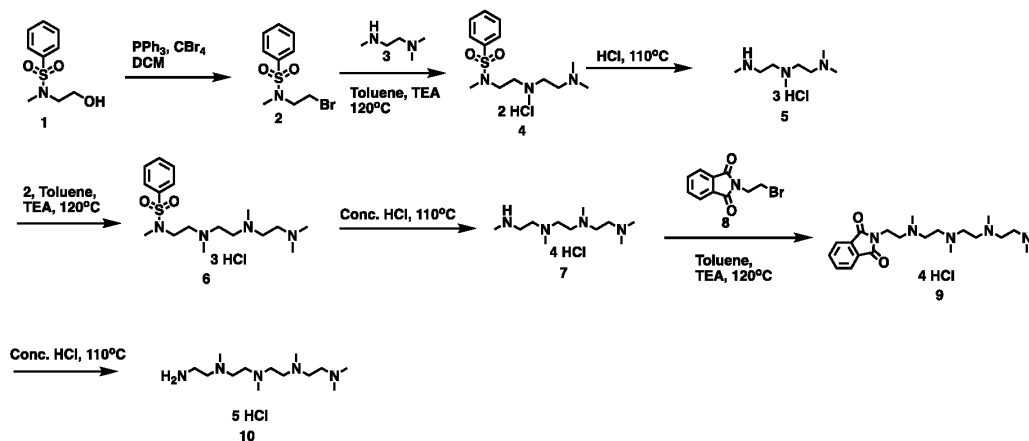
Scheme 5: Synthesis of Amine Compound 10
