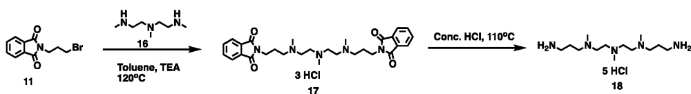
Scheme 17: Synthesis of Polymer J
