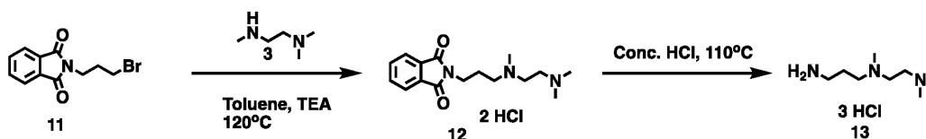
Scheme 7: Synthesis of Amine Compound 13
