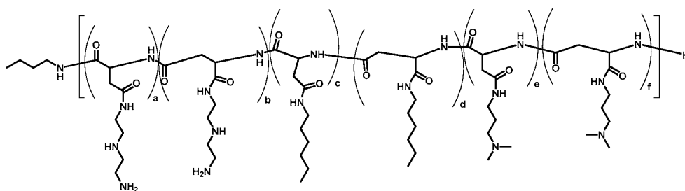
Polymer 52
