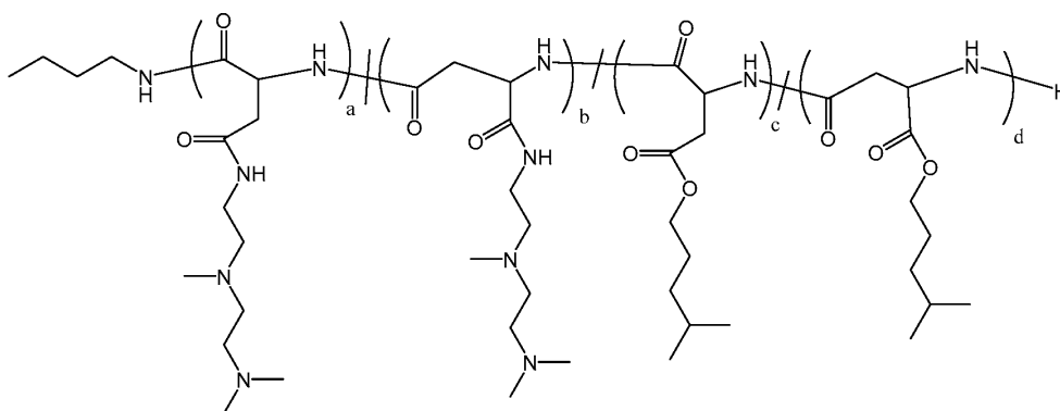
Polymer 36
