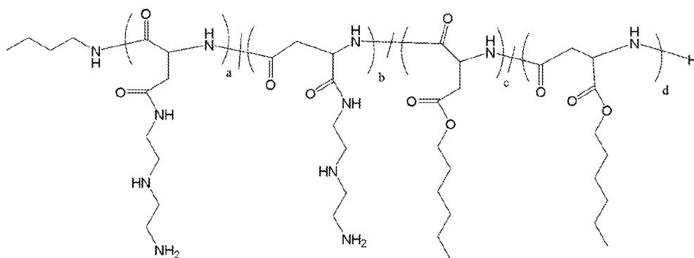
Polymer 14
