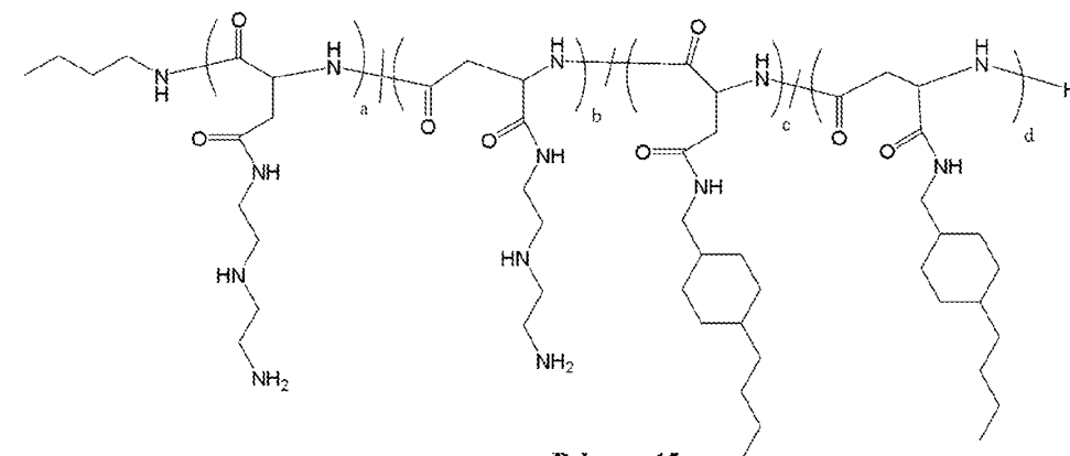
Polymer 15
