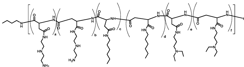
Polymer 53
