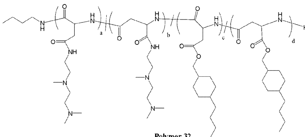
Polymer 32
