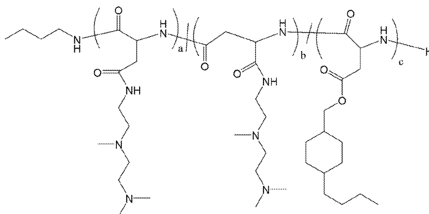
Polymer 26
