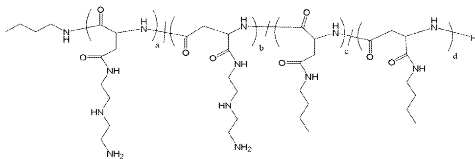
Polymer 11
