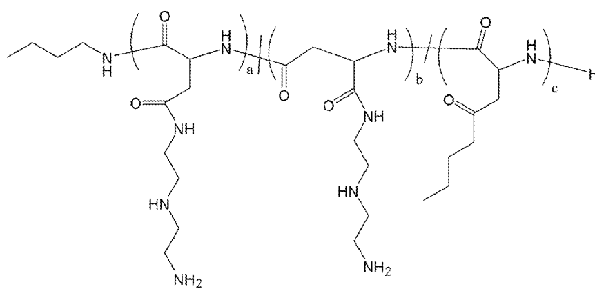
Polymer 6
