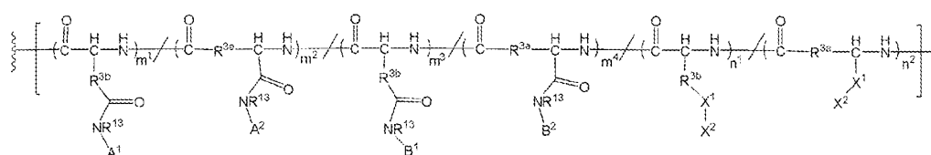
Formula 4
