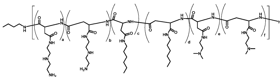
Polymer 44
