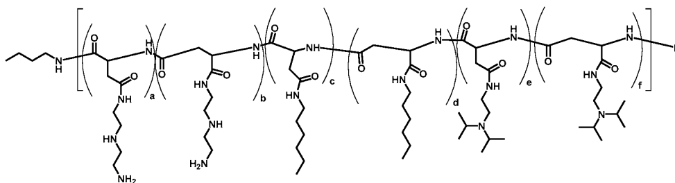
Polymer 46
