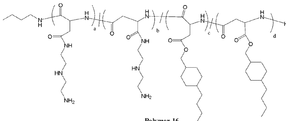
Polymer 16
