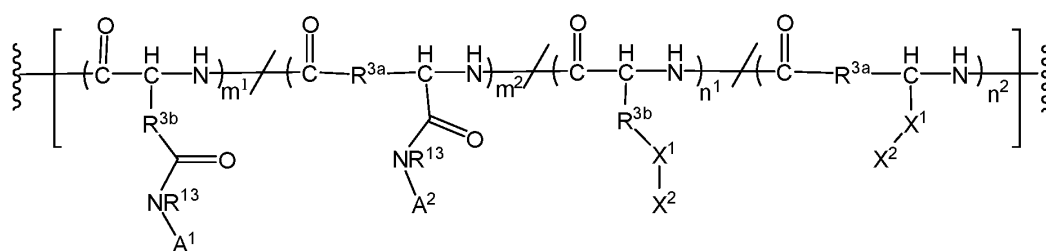
Formula 4
