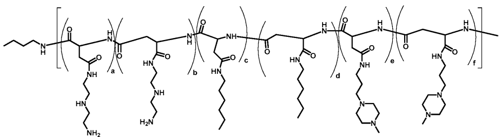
Polymer 57
