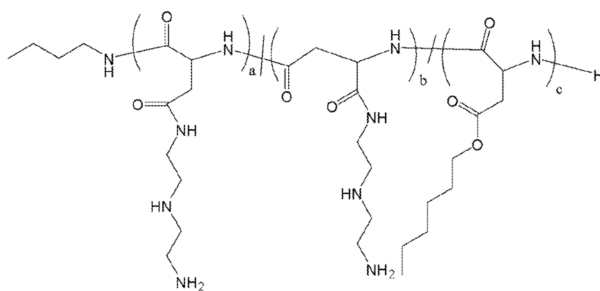
Polymer 4
