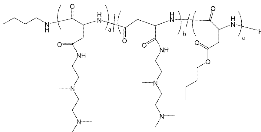
Polymer 24
