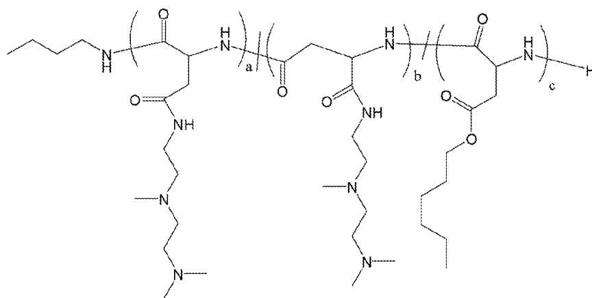
Polymer 20
