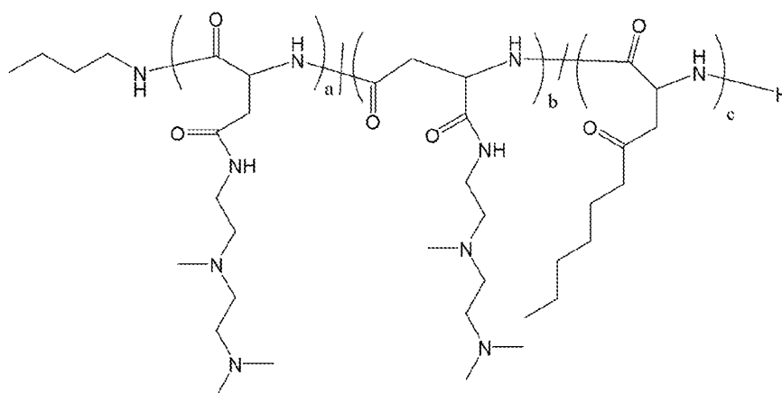
Polymer 18
