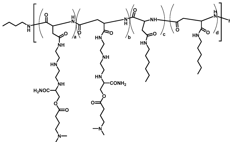
Polymer 64
