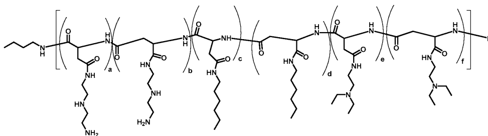
Polymer 45
