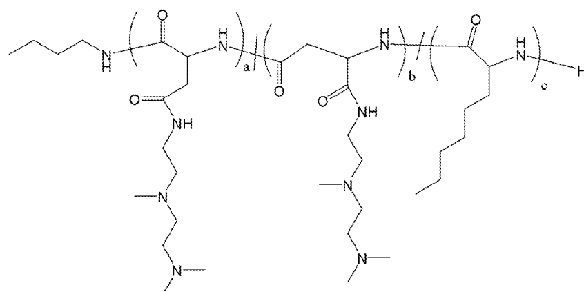
Polymer 17
