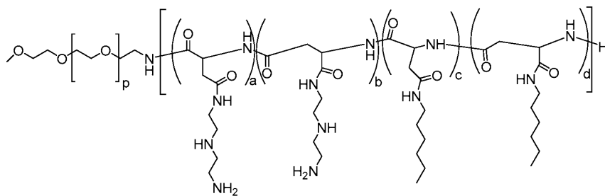
Polymer 68
