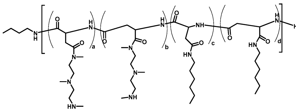
Polymer 40
