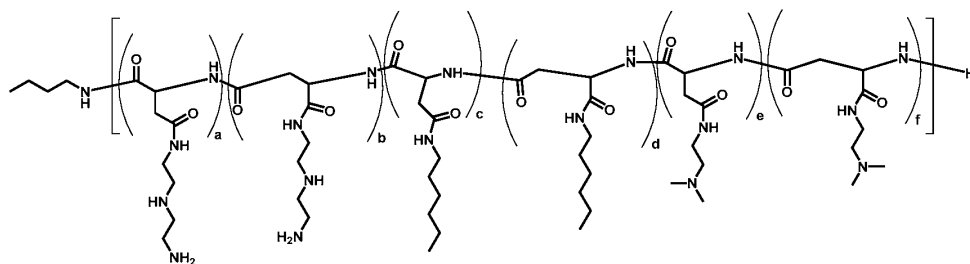
Polymer 44
