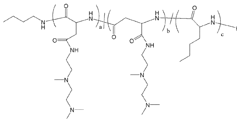
Polymer 21
