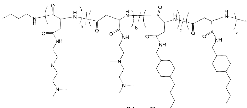
Polymer 31
