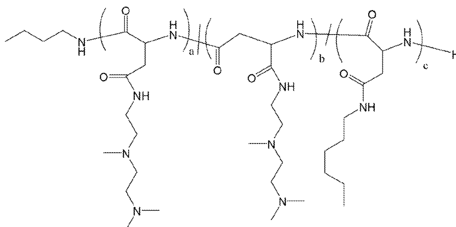
Polymer 19
