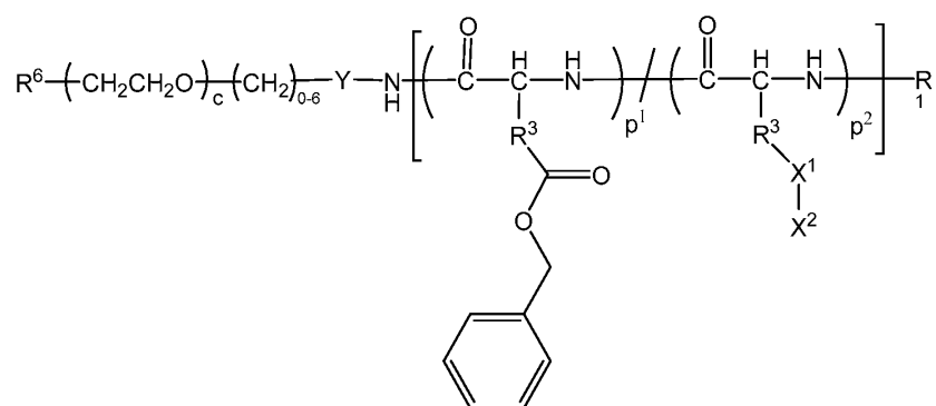
Formula 3A
