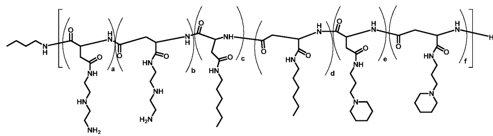
Polymer 55
