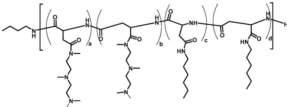
Polymer 39
