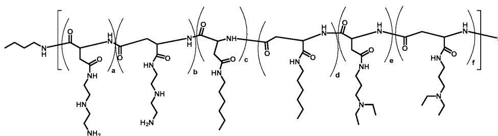
Polymer 53
