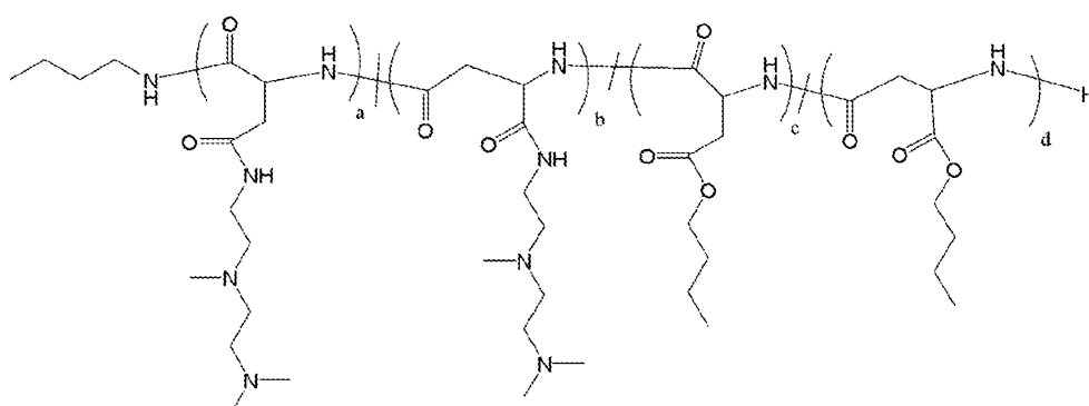
Polymer 28
