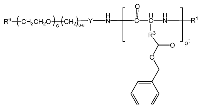
Formula 2A
