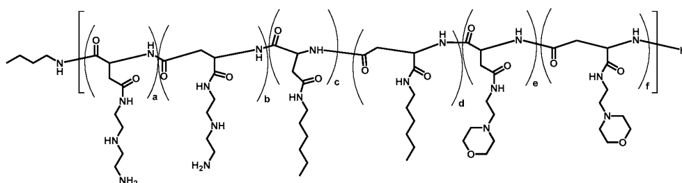
Polymer 48
