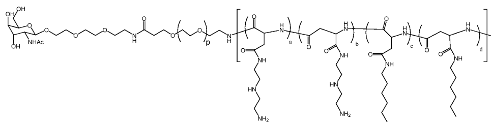
Polymer 69
