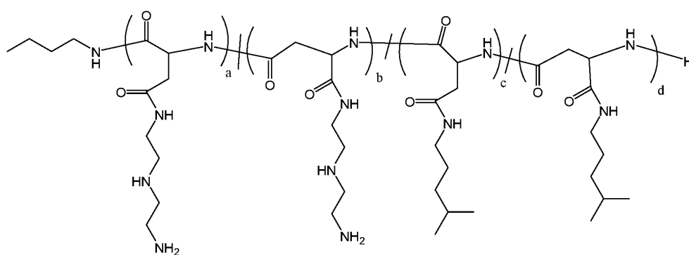
Polymer 33
