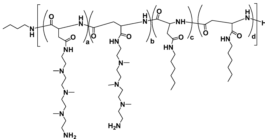
Polymer 42
