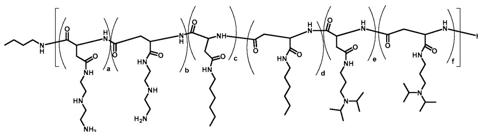
Polymer 54
