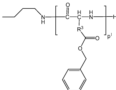
Formula 2B
