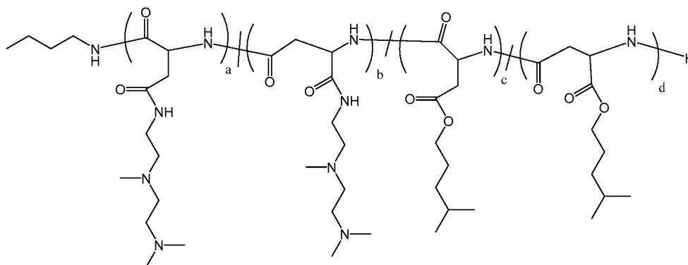
Polymer 36
