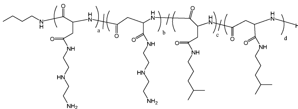
Polymer 33
