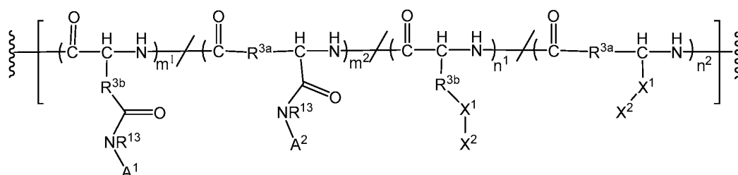
Formula 4
