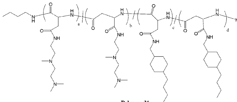
Polymer 31
