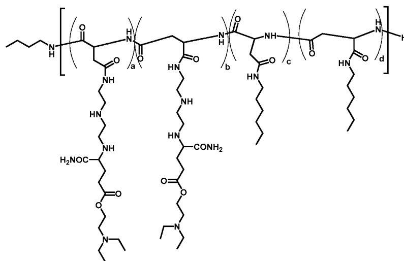
Polymer 63
