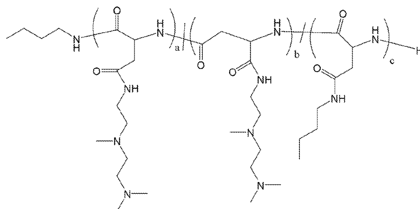
Polymer 23
