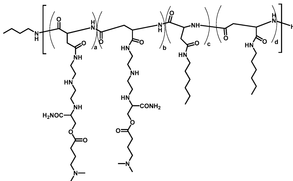
Polymer 64
