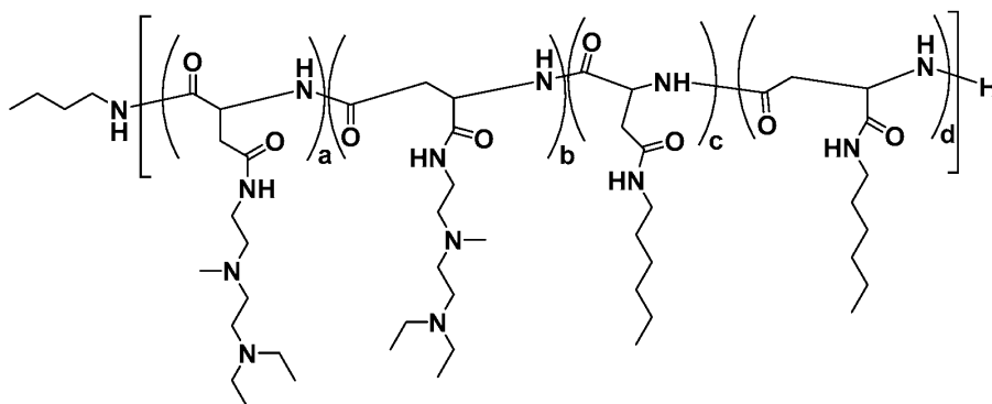
Polymer 43
