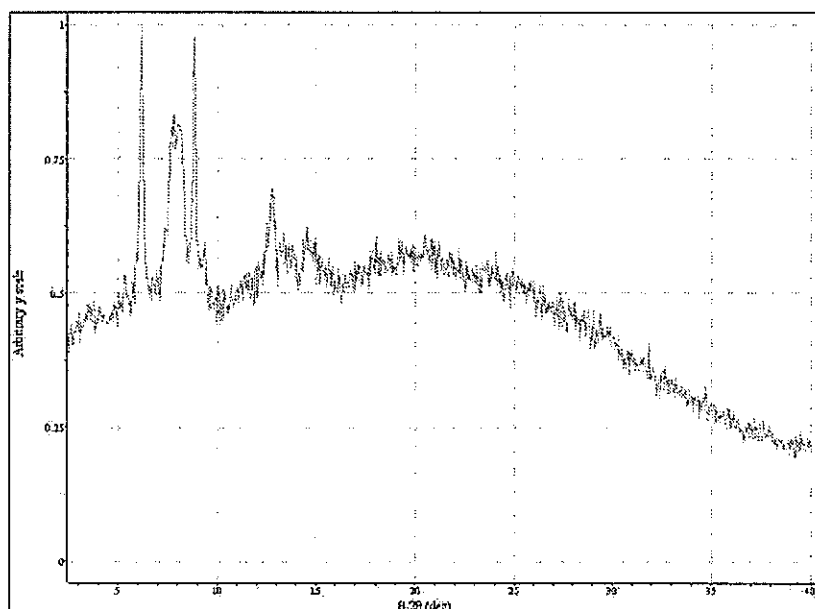
XRPD Pattern of Rifaximin Form \eta
