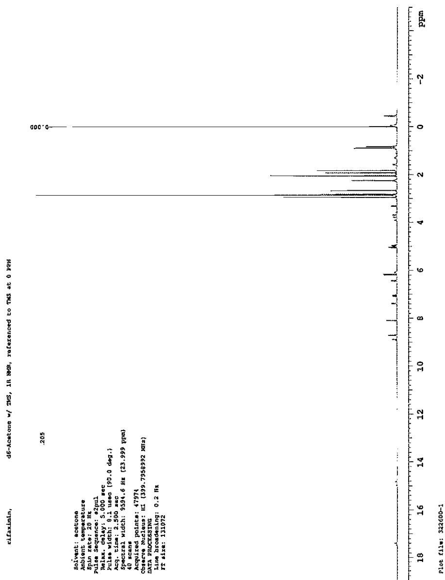
Proton NMR spectrum of Rifaximin, Form \epsilon
