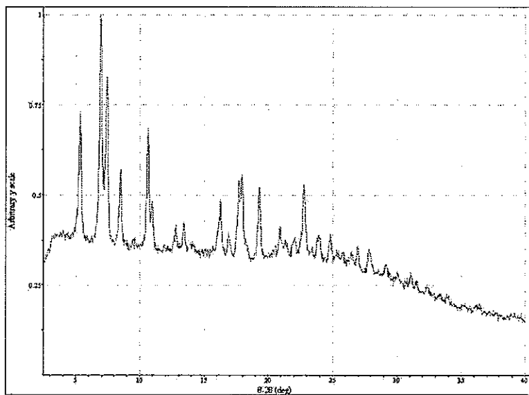
XRPD pattern of Rifaximin Mesylate Salt.
