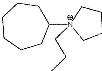
N-propyl-N-cycloheptylpyrrolidinium cation
