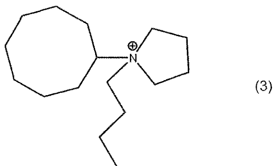
N-butyl-N-cyclooctylpyrrolidinium cation
