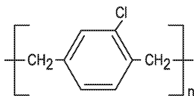
Parylene C
