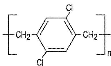
Parylene D
