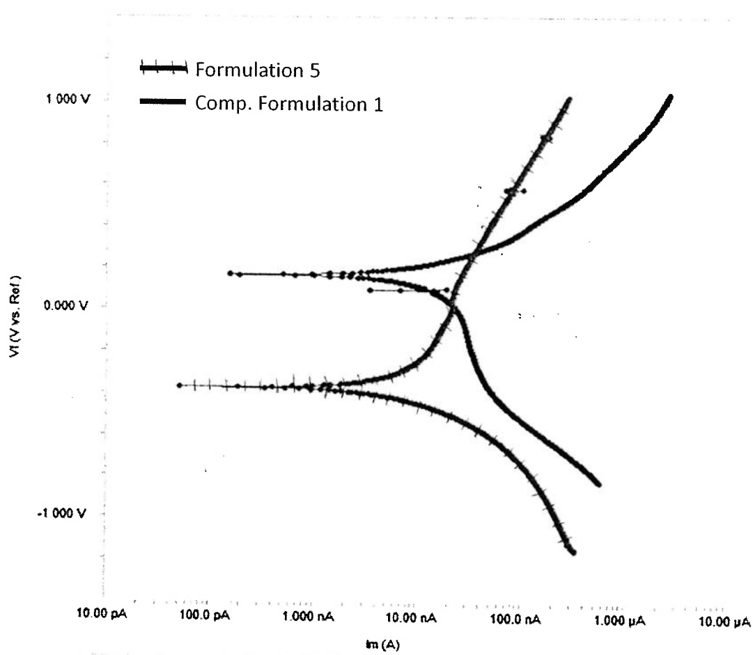
Figure 1. Tafel plot for Formulation 5 and Comparative Formulation 1.
