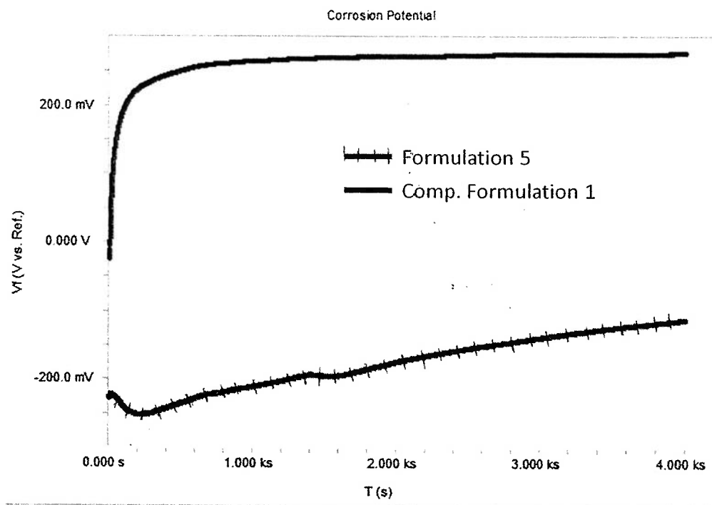
Figure 2. Open circuit potential for Formulation 5 and Comparative Formulation 1.
