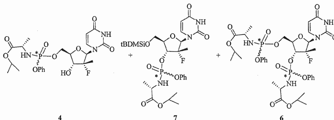
3'-O-phosphoramidate-5'-O-tBDMS (2 diastereomers)
