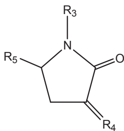
Formula II
