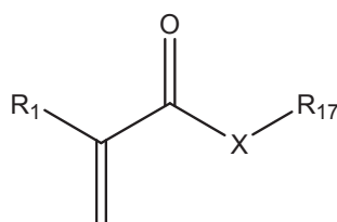
FORMULA IX
