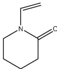
Formula V
