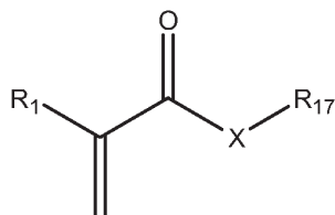
FORMULA IX
