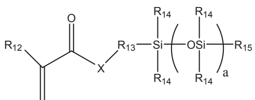
Formula VII
