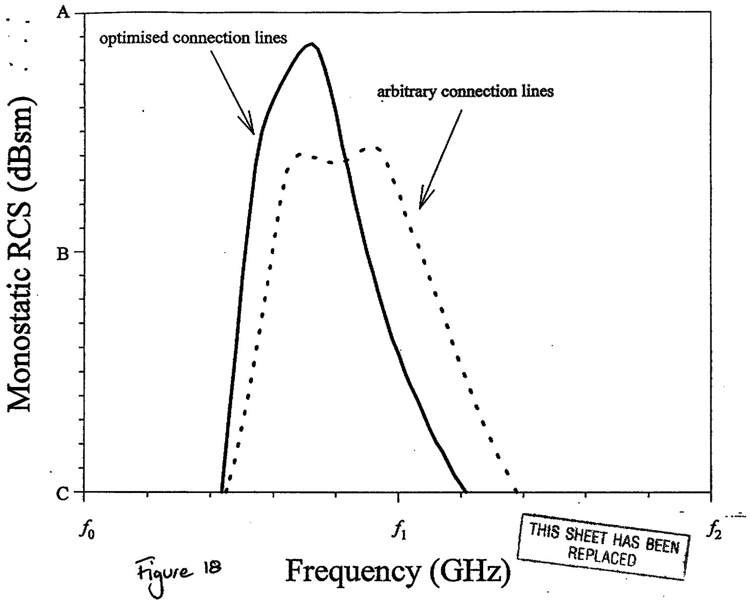
Fig 5.2 Results of arbitrary connection lines
