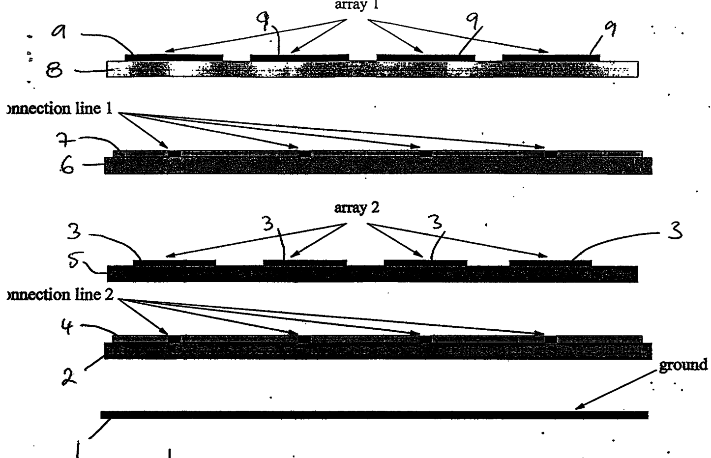
Fig.10 Current invention using stacked arrays
