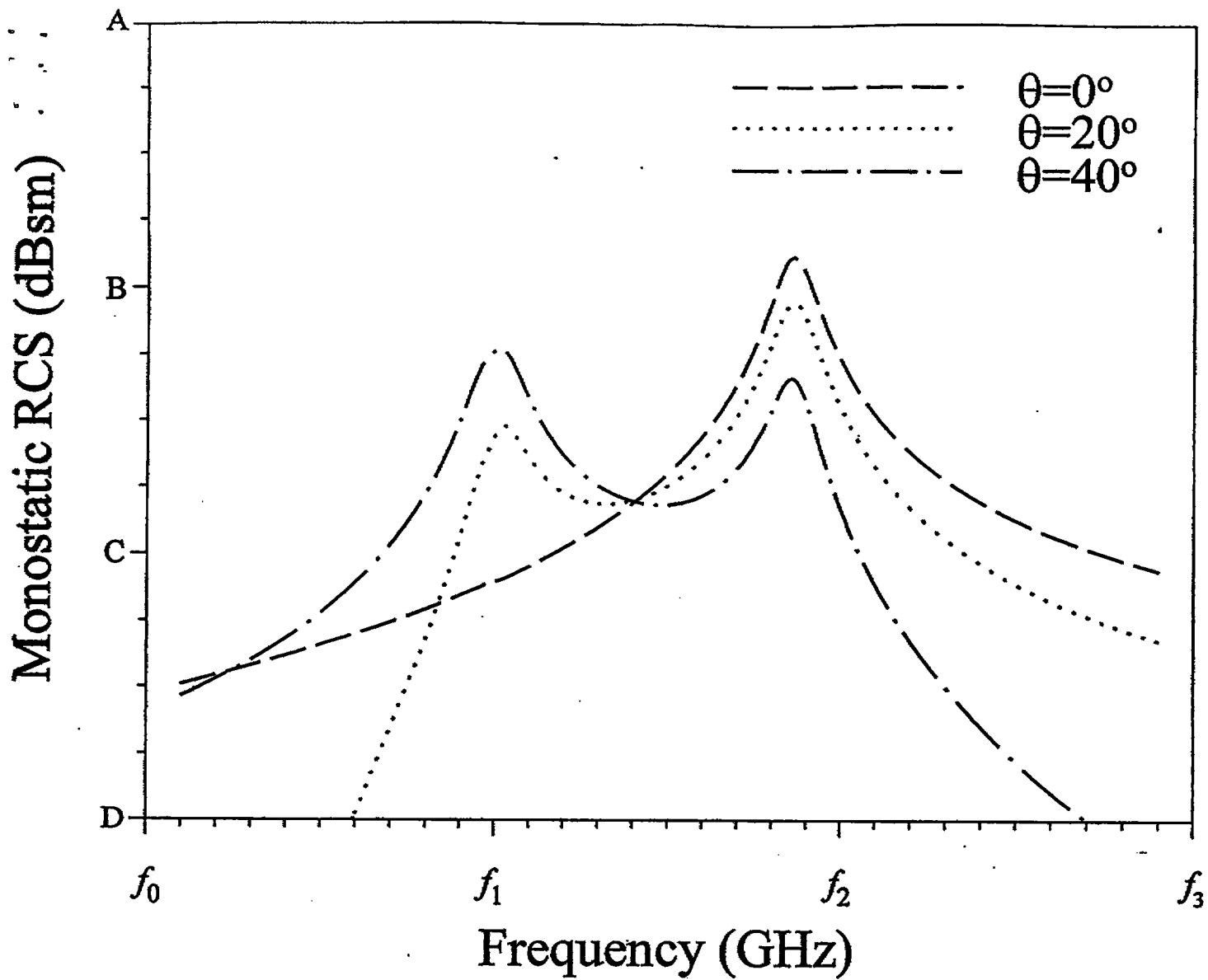
Fig. 6.2 Results of Van Atta array with directed connection lines
