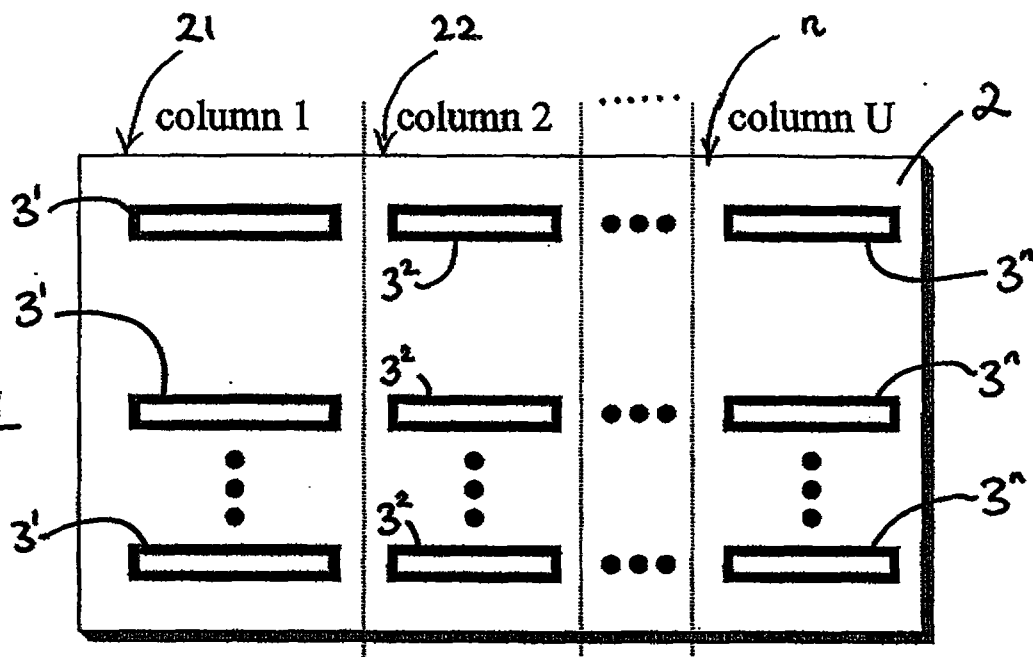
Figure 29 Current invention using multi-frequency rectangular loops.
