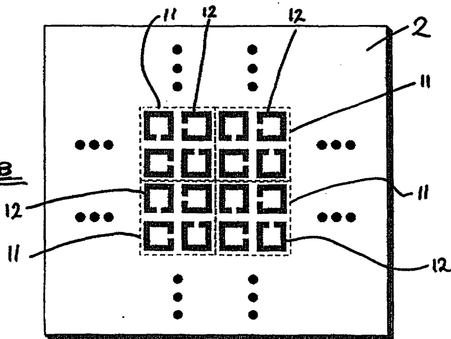
Figure 28 Current invention using unit cells containing four sequential rotated C-type radiating elements.
