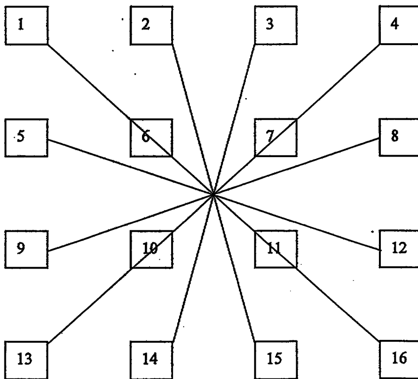
Figure 1.1: Van Atta Array
