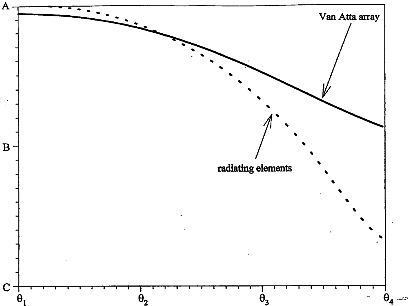
Figure 10 \theta (degree) Fig 3.2 Results of Van Atta array and radiating elements
