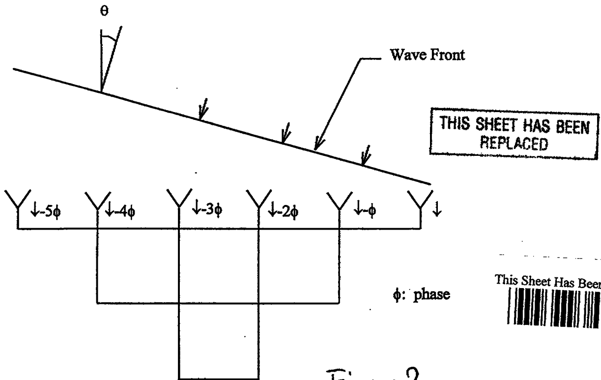
Figure 1.1: Van Atta Array
