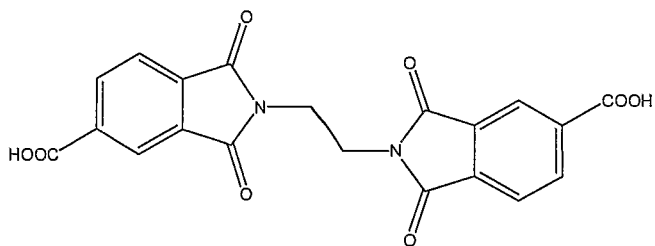
(TMA-EDA imide)
