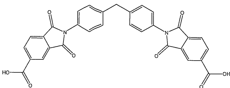
(TMA-MDA imide)
