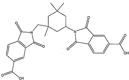
(TMA-IPDA imide)
