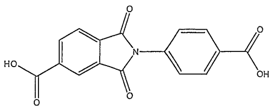
(TMA-PABA imide)
