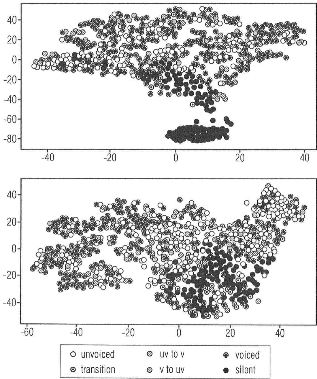
t-SNE projection of latent frames for voicing information
