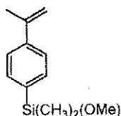
α-methylstyryl dimethylmethoxysilane
