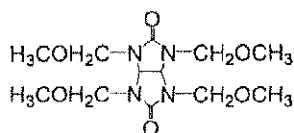
NIKALAC MX-270
