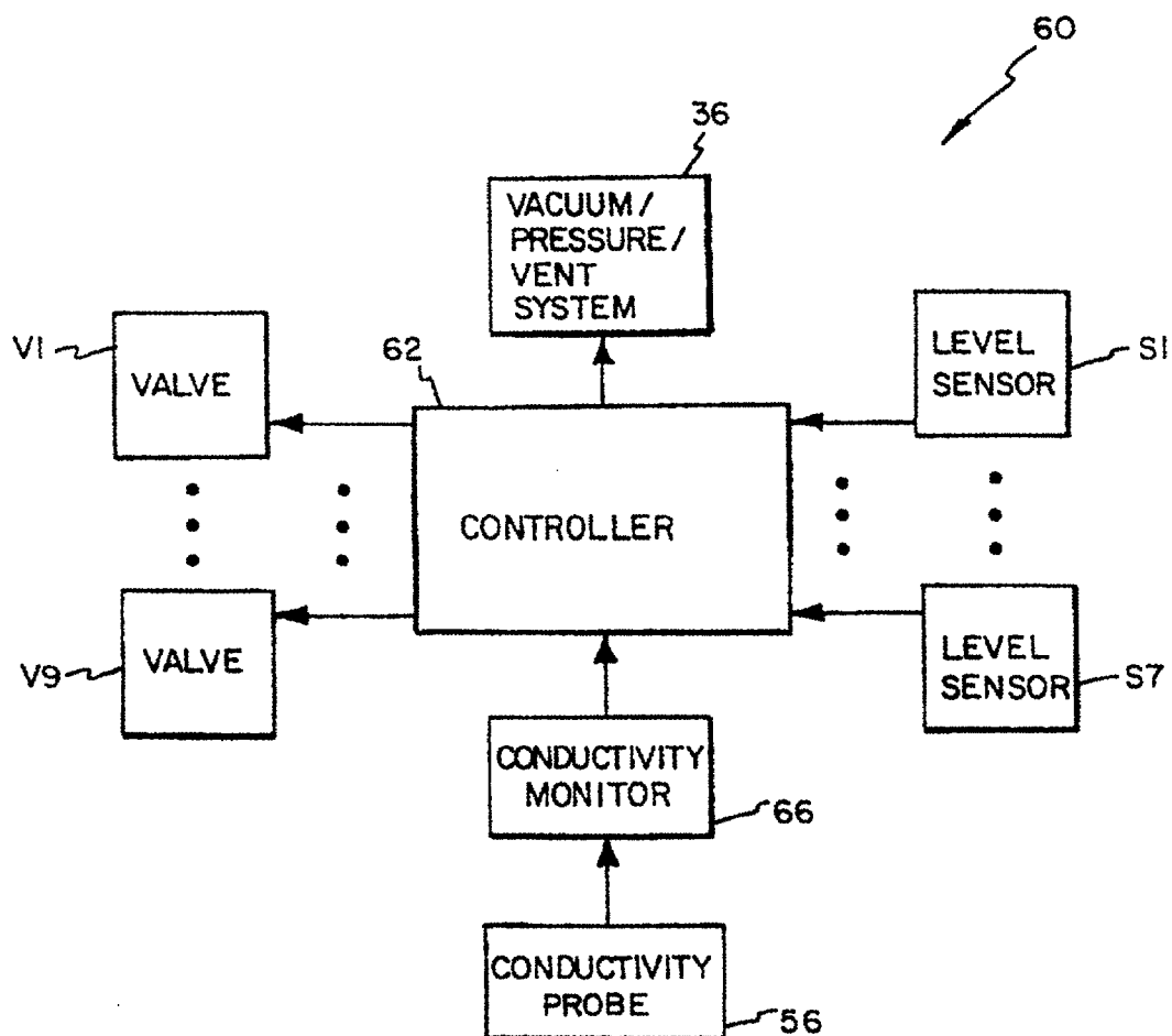
CONTROL SYSTEM 60
