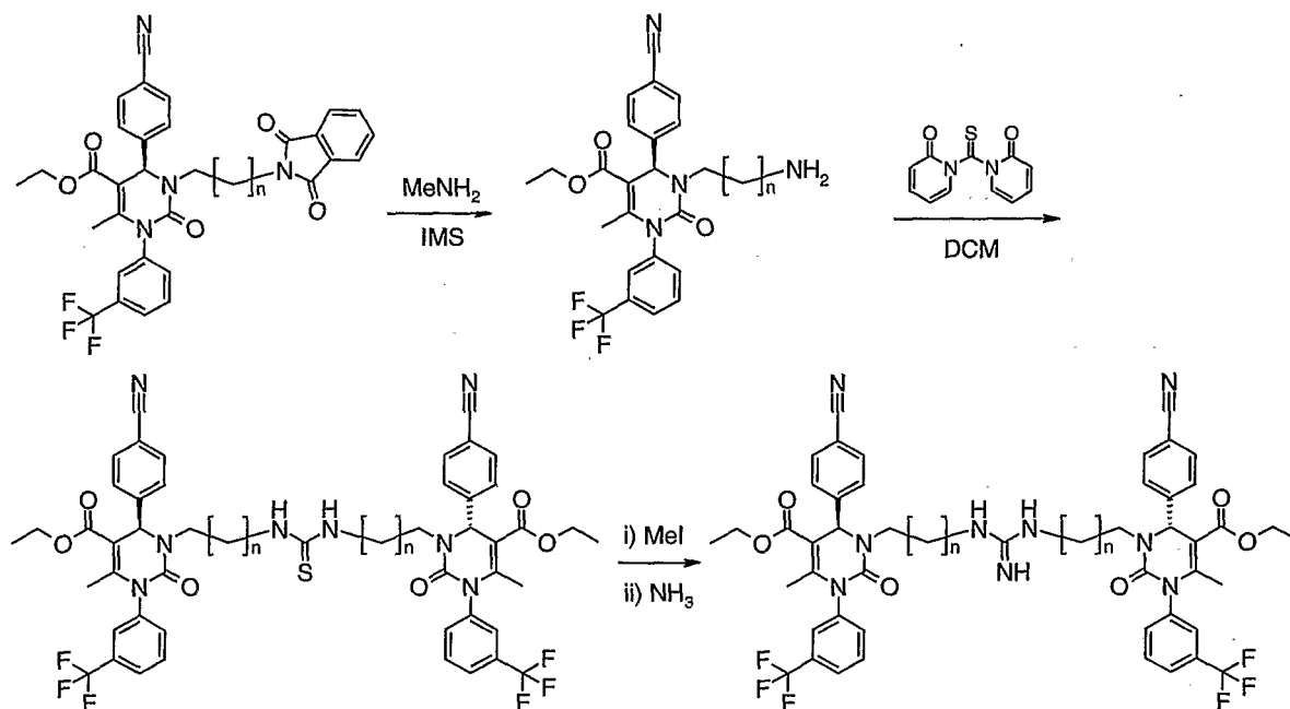
5 Scheme 6
