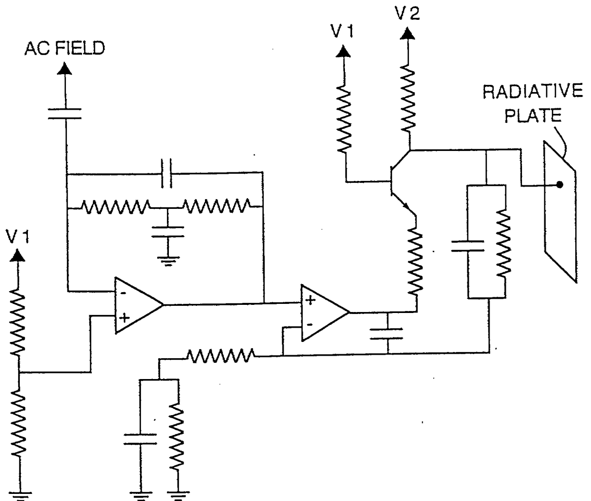
FIG. 1 (PRIOR ART)
