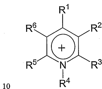
Pyridinium
