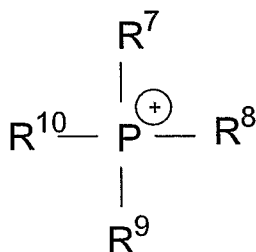
Phosphonium
