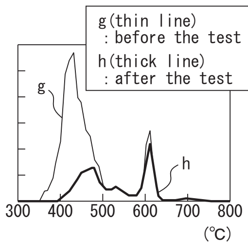
(2) GCD curve of the lubricant composition of Reference Example 2
