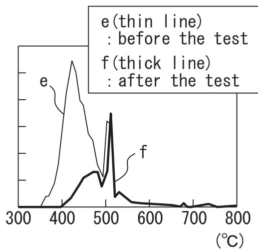
(1) GCD curve of the lubricant composition of Reference Example 1
