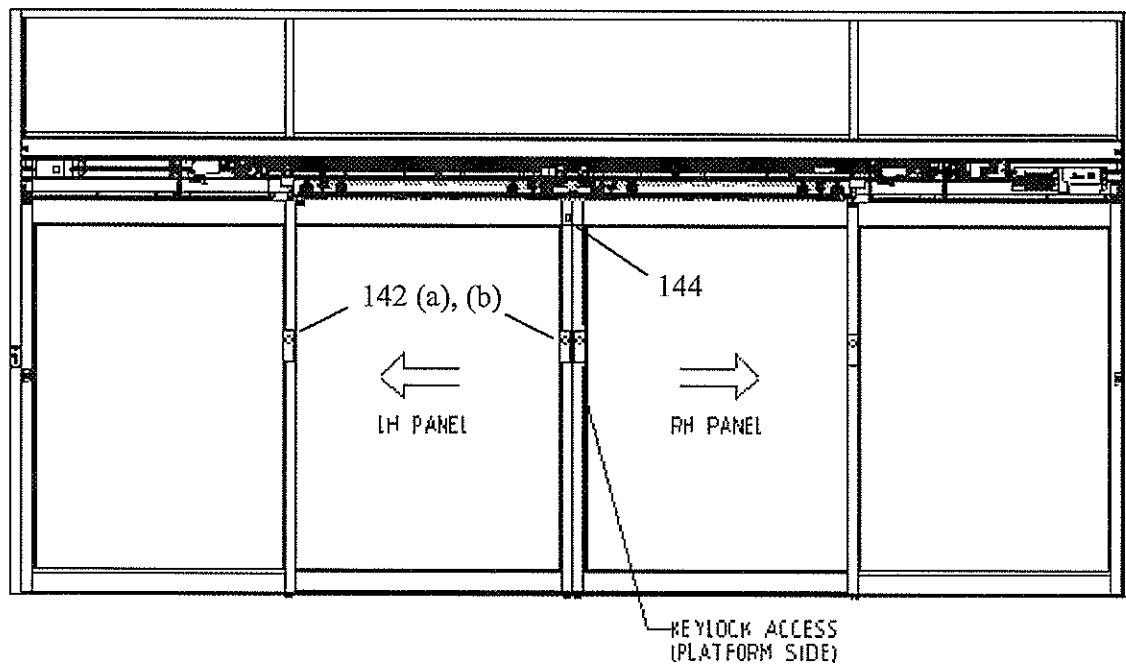
PLATFORM SIDE ELEVATION
