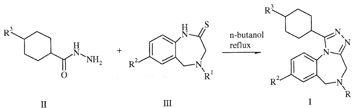
Scheme 1: General Scheme A
