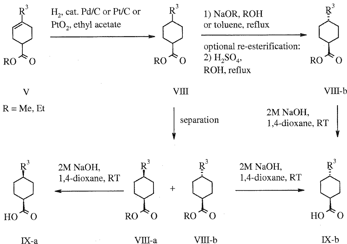
Scheme 5: General Scheme E
