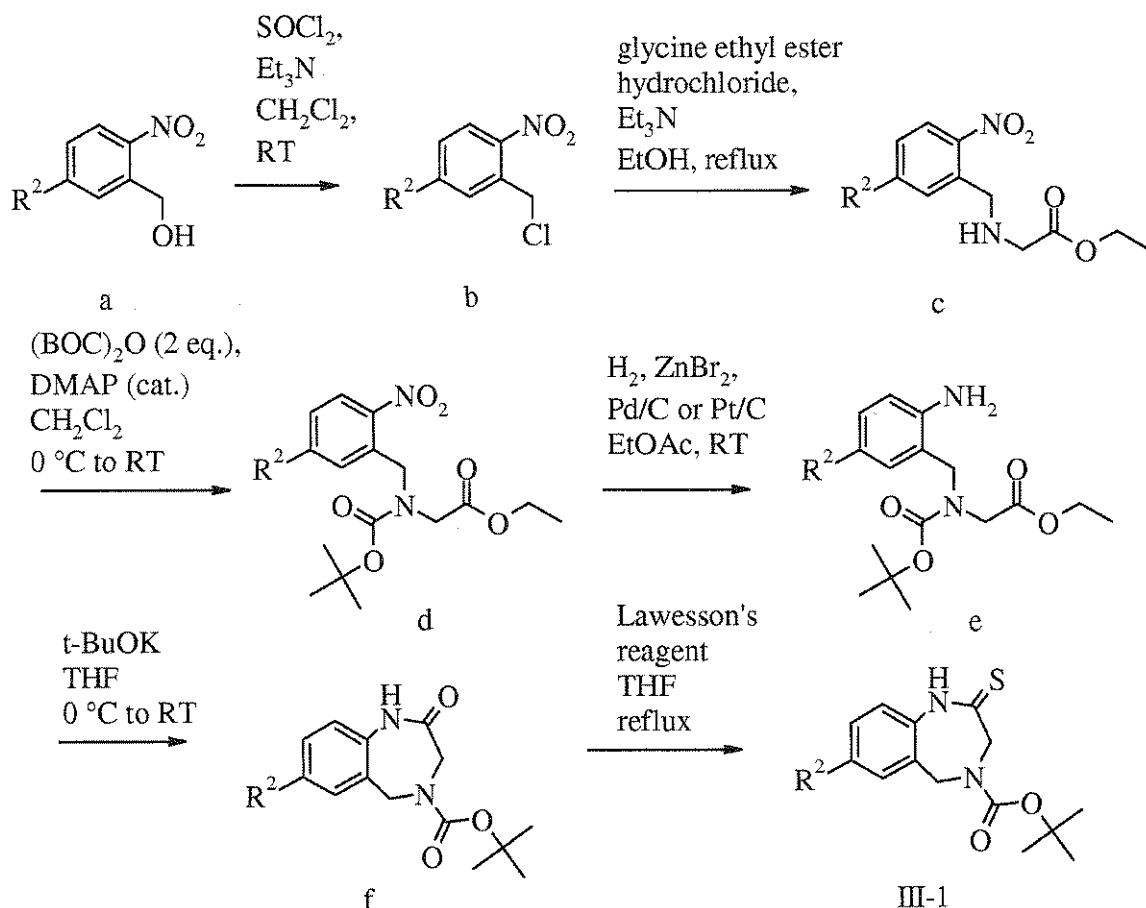
Scheme 3: General Scheme C
