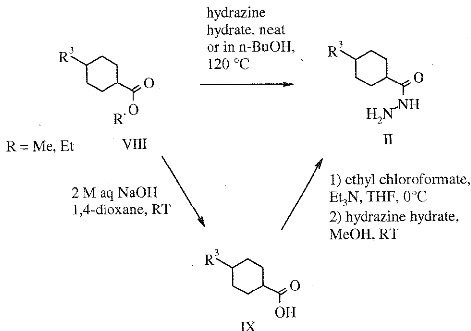
Scheme 6: General Scheme G
