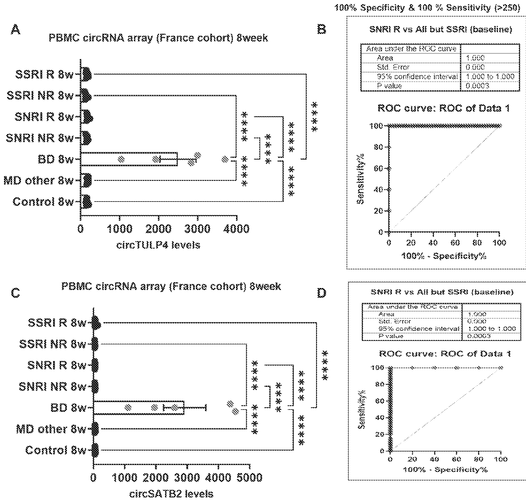
Figure 15: 8 week BD diagnosis prediction based on circTULP4 or circSATB2 (circRNA array profiling from 100 PBMC samples from the France cohort)
