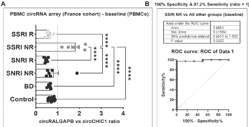
Figure 12: Baseline SSRI remission prediction based on 2 circRNAs (circRNA array profiling from 100 PBMC samples from the France cohort)
