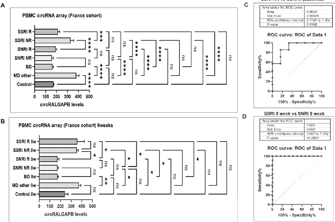
Figure 7: SSRI remission and SSRI vs SNRI treatment predictions based on circRAGAPB levels (circRNA array profiling from 100 PBMC samples from the France cohort)
