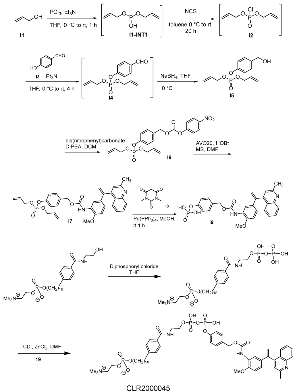
Scheme 4
