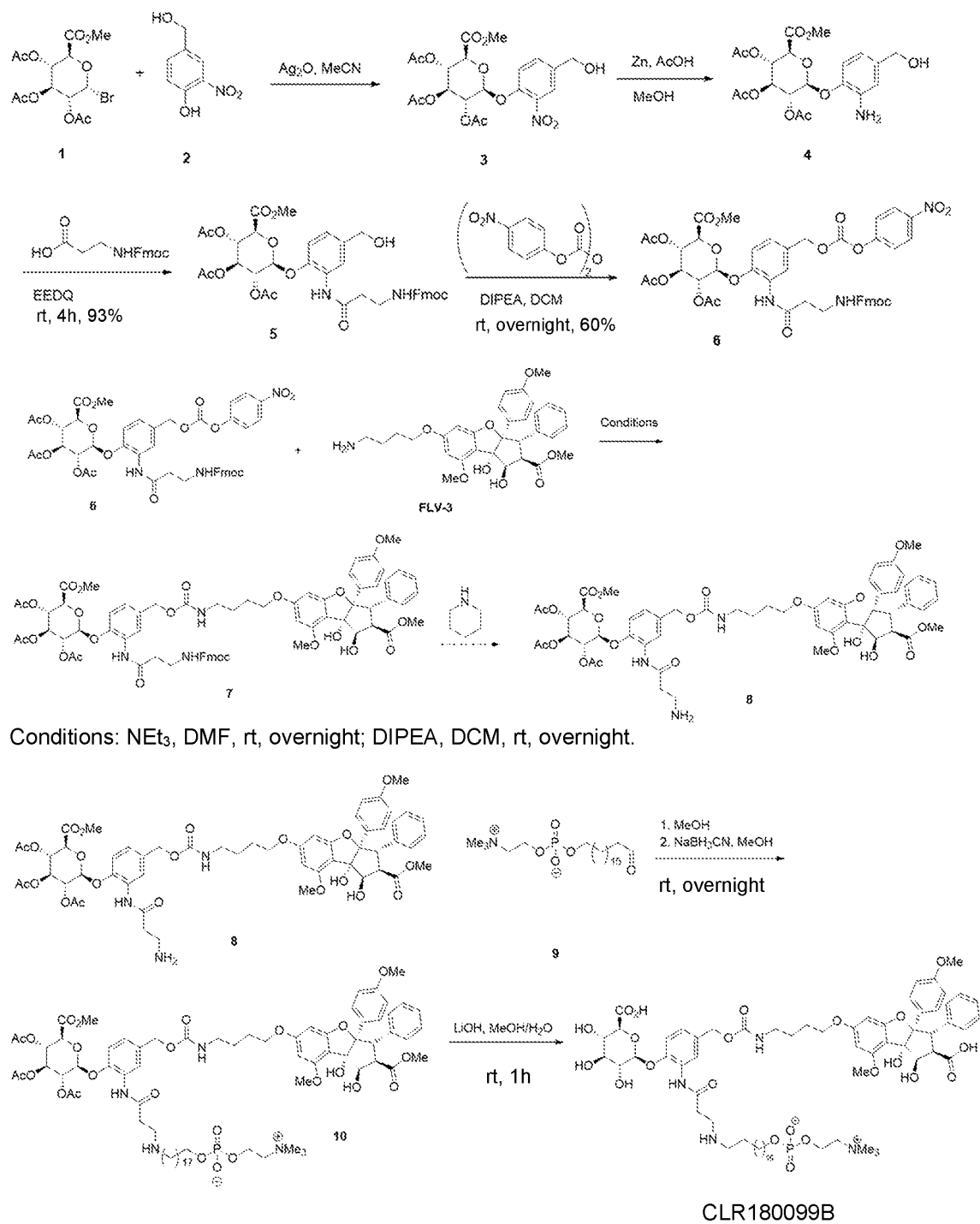
Scheme 8
