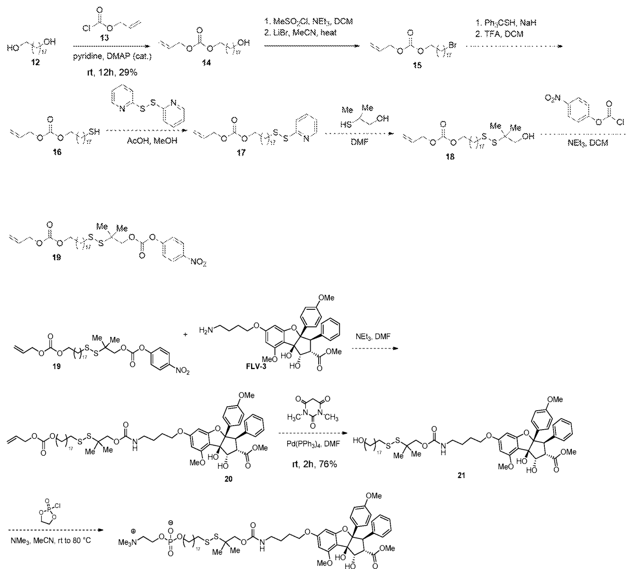
Scheme 7
