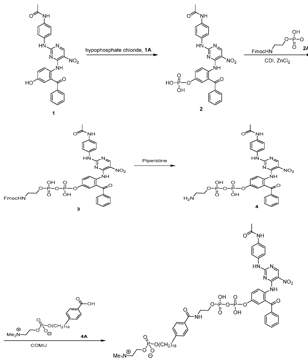
Scheme 2
