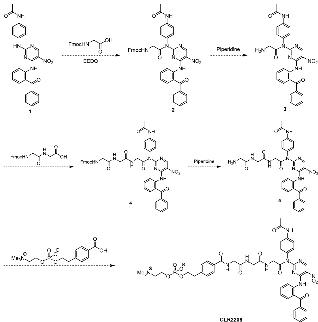
Scheme 1
