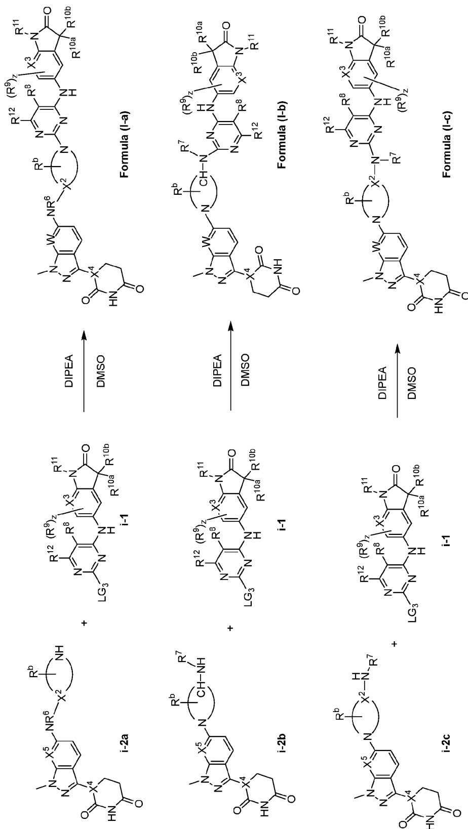
Scheme 4.
