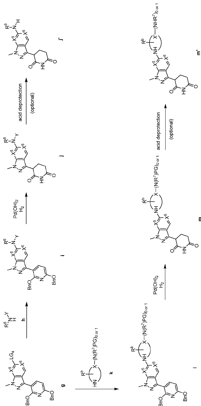
Scheme 2.
