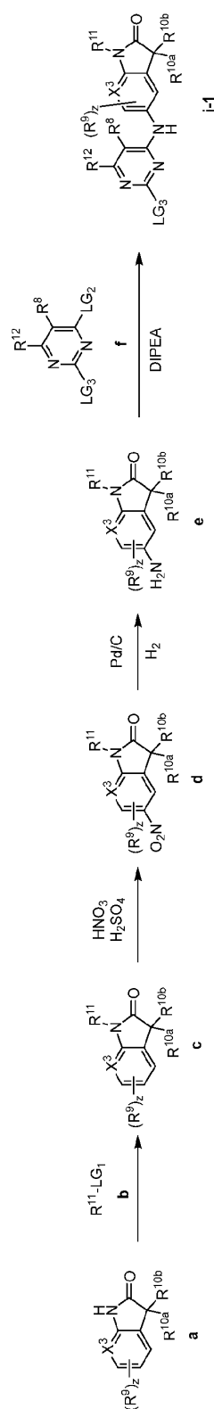
Scheme 1.
