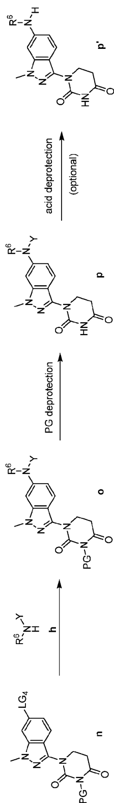
Scheme 3.
