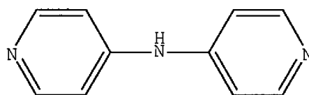
dipyrindin-4-ylamine
