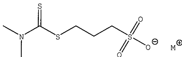
Structure (5)
