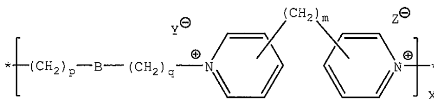
Structure (IV)
