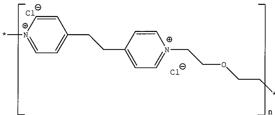
Structure (VIII)
