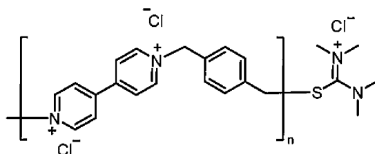
Structure D
