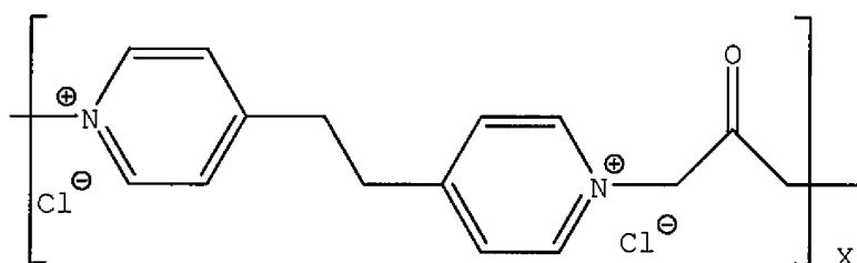
Structure (X)
