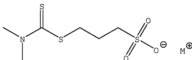
Structure (5)
