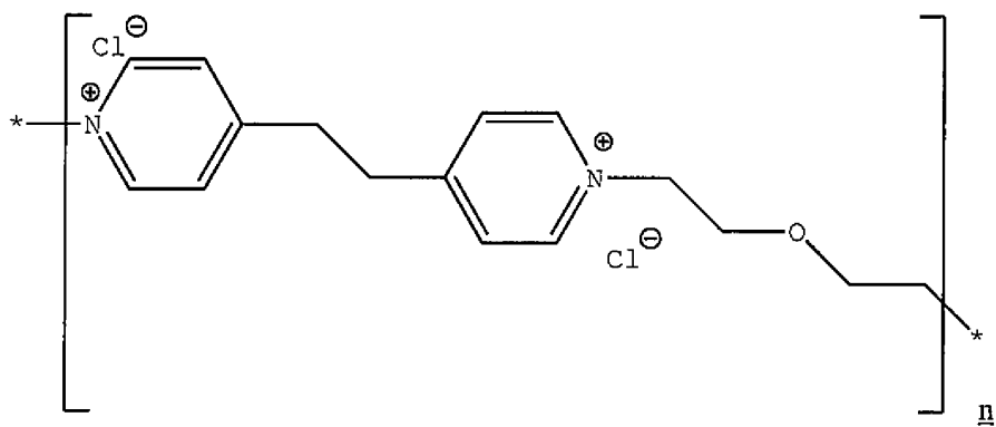
Structure (VIII)
