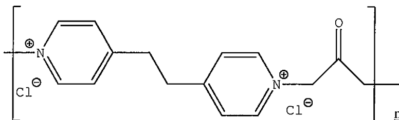
Structure (X)
