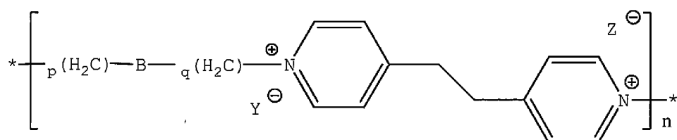
Structure (VII)
