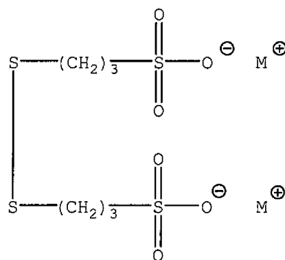
Structure (2)
