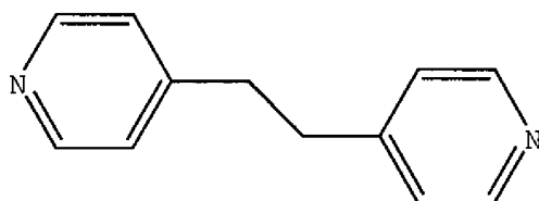
Structure (IIf)
