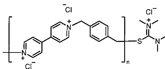
Structure D.
