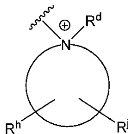
(2B)
