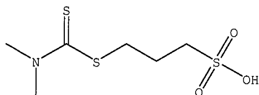
Structure (16)
