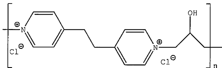
Structure (XI)
