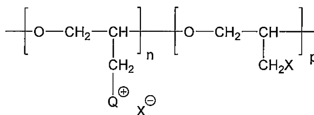
(IC)
