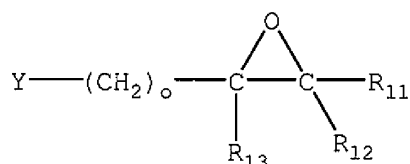
Structure (IIIc)
