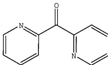
2,2'-dipyriddy ketone
