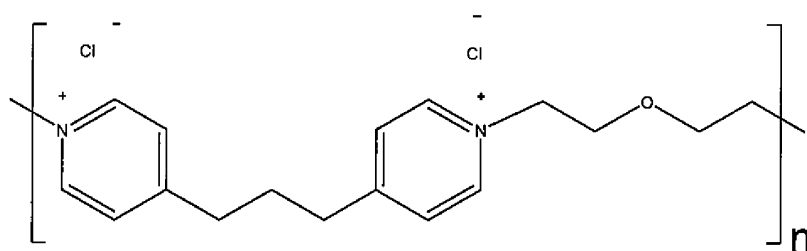
Structure (XXX)
