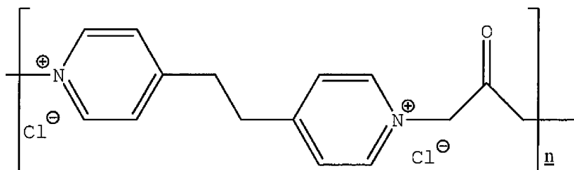
Structure (X)
