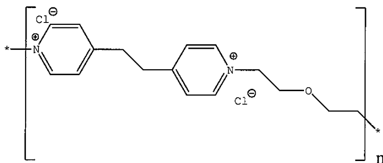
Structure (VIII)
