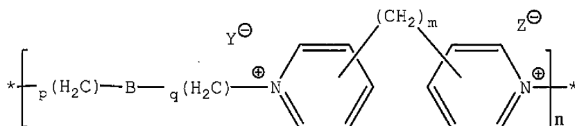
Structure (IV)
