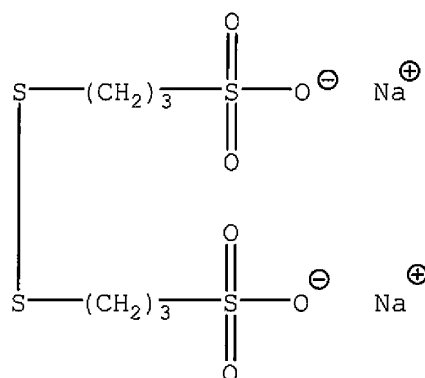
Structure (3)
