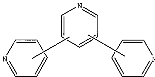
Structure (Id)
