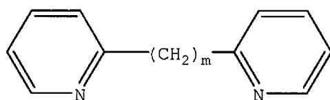
Structure (IIb)
