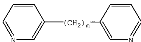
Structure (IIc)
