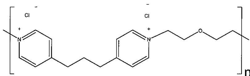
Structure (XXX)
