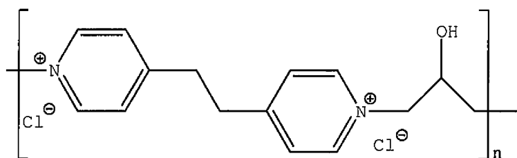
Structure (XI)
