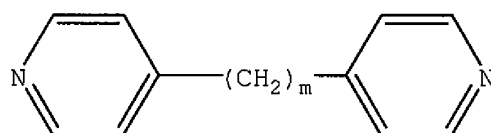
Structure (IIe)
