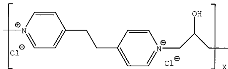
Structure (XI)
