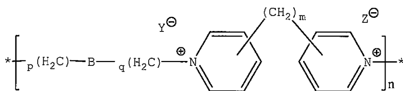
Structure (IV)
