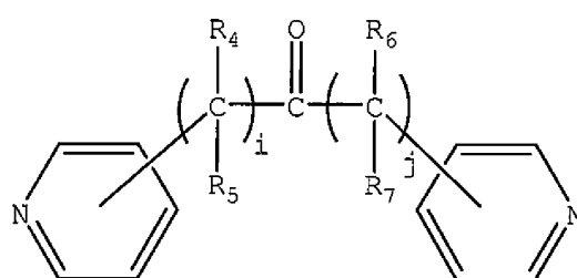
Structure (Ib)
