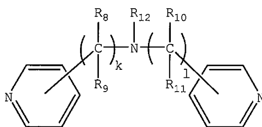
Structure (Ic)
