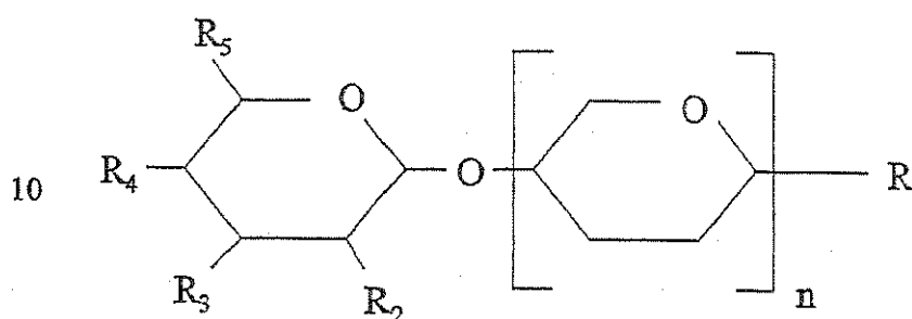
Fig.1. Polymeric acid oligosaccharide
