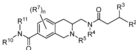
Formula (Ig);
