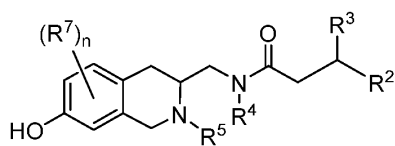
Formula (Ih);
