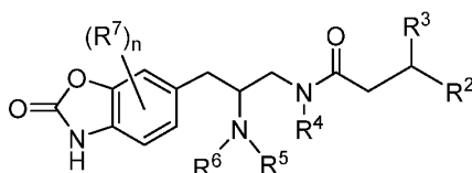
Formula (Id);
