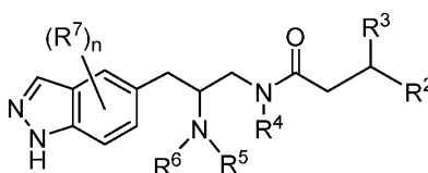
Formula (Ic);
