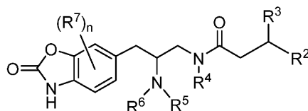
Formula (Id);
