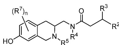
Formula (Ih);
