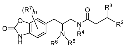
Formula (Id);
