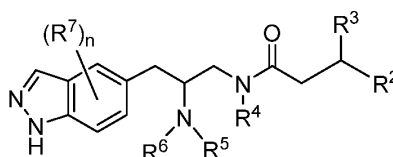
Formula (Ic);
