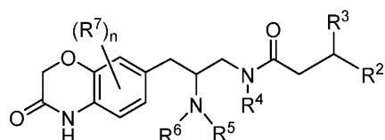
Formula (If);
