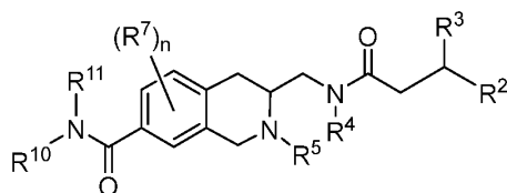
Formula (Ig);
