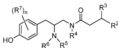
Formula (Ib);
