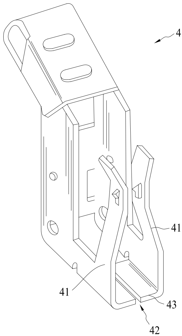
FIG. 2 (Prior Art)
