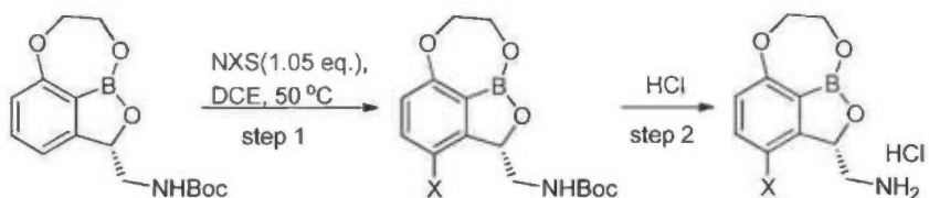
[0085] Scheme 4
