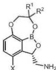
Formula IIa
