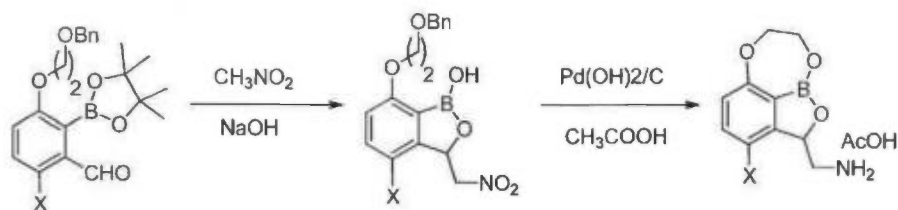
[0083] Scheme 3
