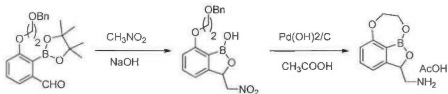
[0083] Scheme 3
